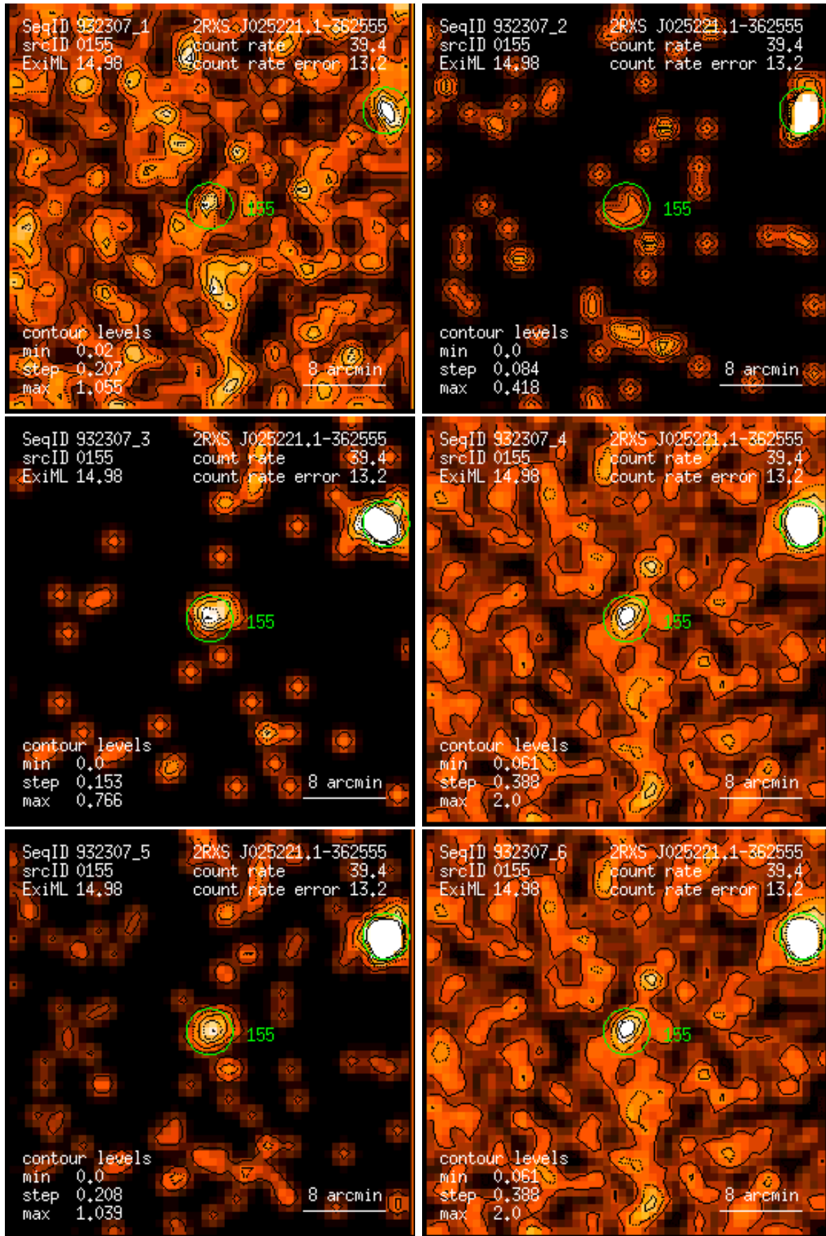
Figure 155: RASS 932307: detection 0155: band rate images, Gaussian filter: (1) PSPC channels 11 – 41, (2) 52 – 90, (3) 91 – 201, (4) 11 – 235, (5) 52 – 201, (6) 11 – 201. Broad band rates in counts/ks. Band rate contour levels in counts/ks/arcmin 2 .
