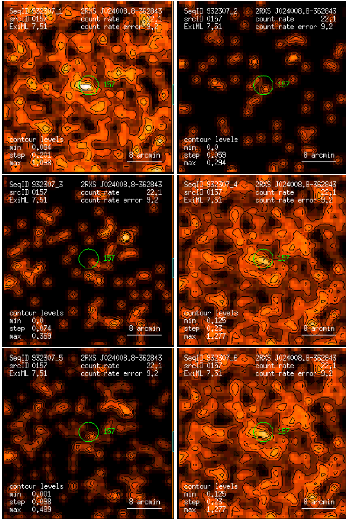
Figure 157: RASS 932307: detection 0157: band rate images, Gaussian filter: (1) PSPC channels 11 – 41, (2) 52 – 90, (3) 91 – 201, (4) 11 – 235, (5) 52 – 201, (6) 11 – 201. Broad band rates in counts/ks. Band rate contour levels in counts/ks/arcmin 2 .
