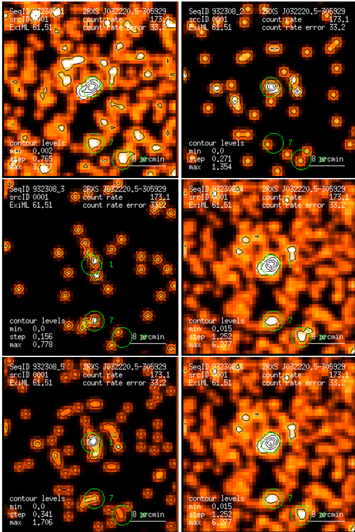
Figure 1: RASS 932308: detection 0001: band rate images, Gaussian filter: (1) PSPC channels 11 – 41, (2) 52 – 90, (3) 91 – 201, (4) 11 – 235, (5) 52 – 201, (6) 11 – 201. Broad band rates in counts/ks. Band rate contour levels in counts/ks/arcmin 2 .
