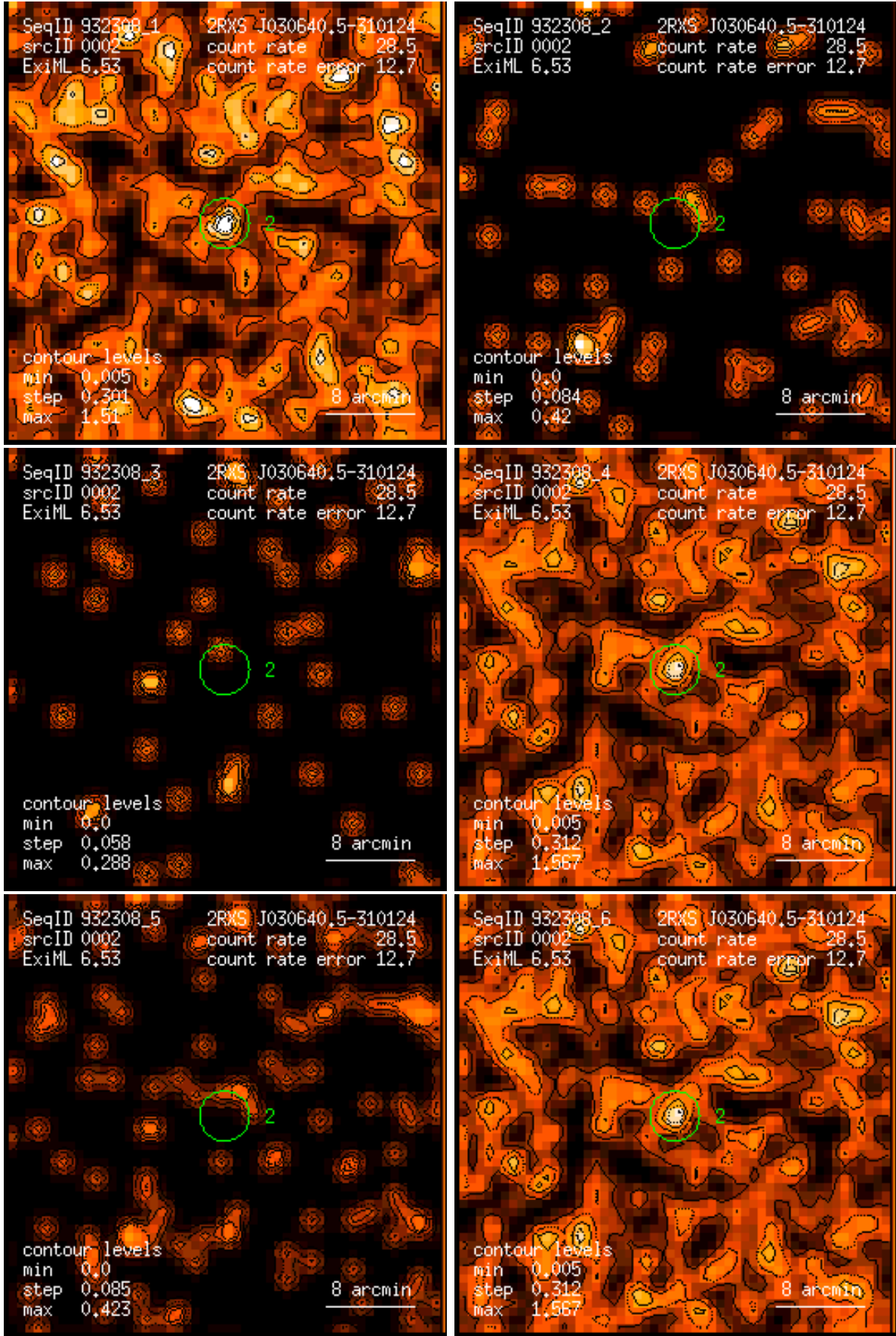
Figure 2: RASS 932308: detection 0002: band rate images, Gaussian filter: (1) PSPC channels 11 – 41, (2) 52 – 90, (3) 91 – 201, (4) 11 – 235, (5) 52 – 201, (6) 11 – 201. Broad band rates in counts/ks. Band rate contour levels in counts/ks/arcmin 2 .
