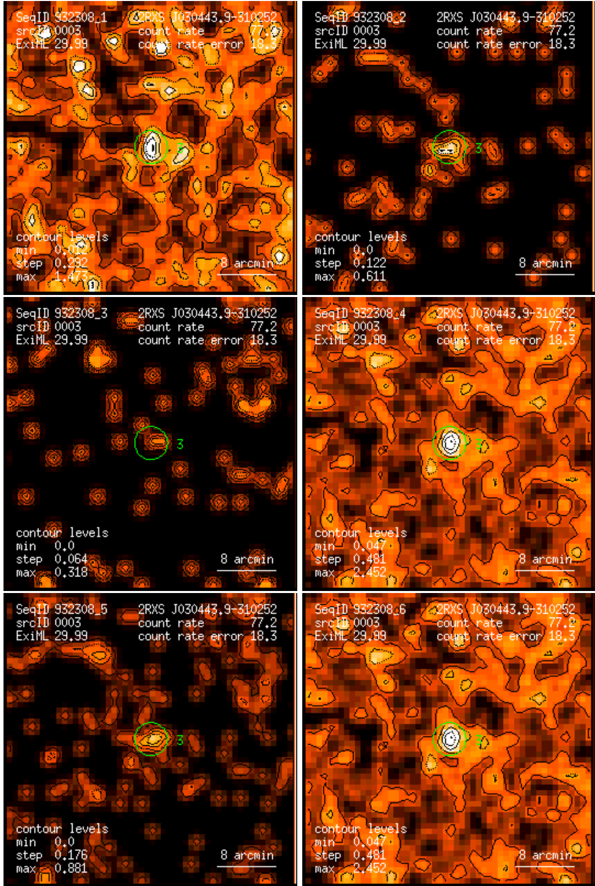
Figure 3: RASS 932308: detection 0003: band rate images, Gaussian filter: (1) PSPC channels 11 – 41, (2) 52 – 90, (3) 91 – 201, (4) 11 – 235, (5) 52 – 201, (6) 11 – 201. Broad band rates in counts/ks. Band rate contour levels in counts/ks/arcmin 2 .
