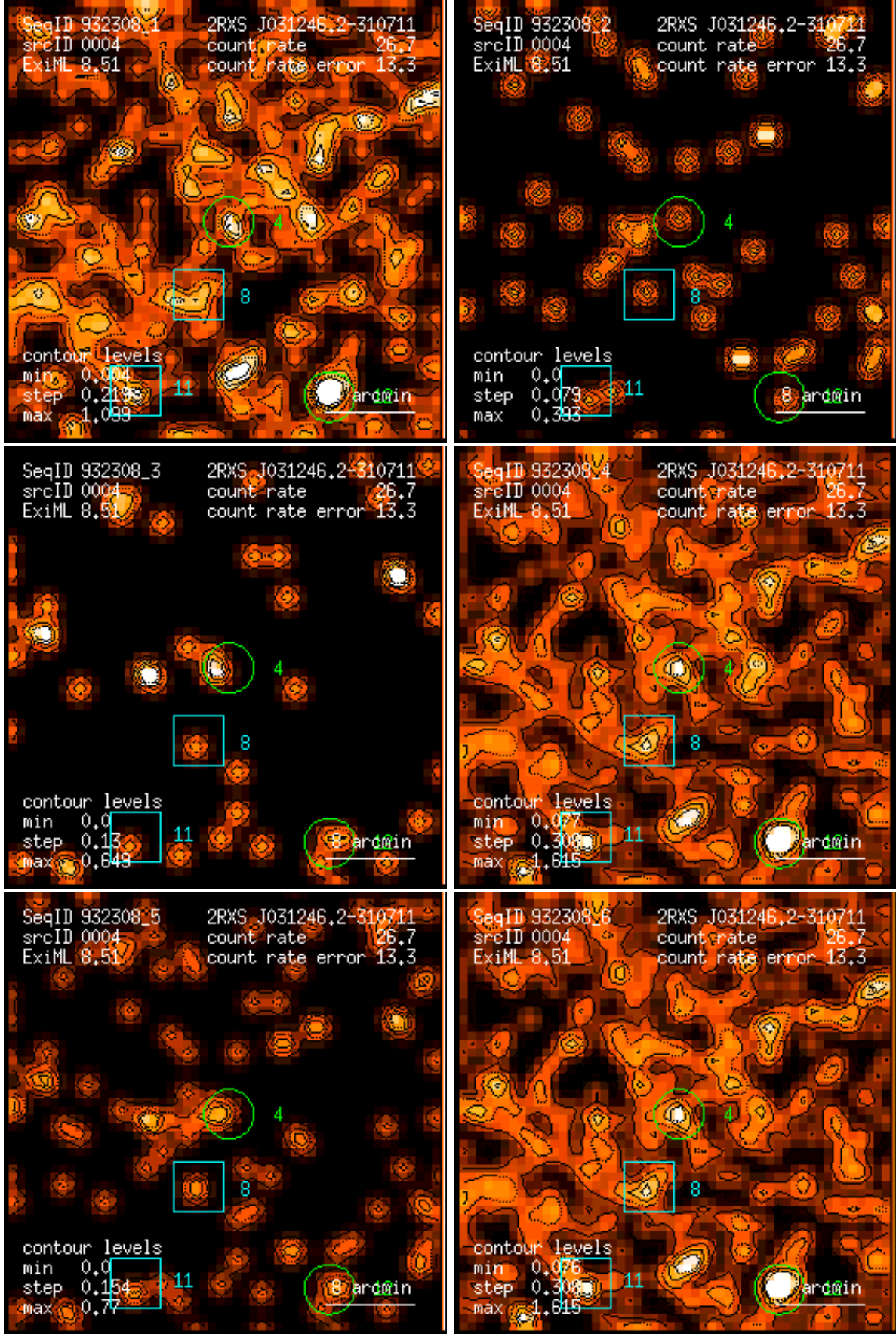
Figure 4: RASS 932308: detection 0004: band rate images, Gaussian filter: (1) PSPC channels 11 – 41, (2) 52 – 90, (3) 91 – 201, (4) 11 – 235, (5) 52 – 201, (6) 11 – 201. Broad band rates in counts/ks. Band rate contour levels in counts/ks/arcmin 2 .
