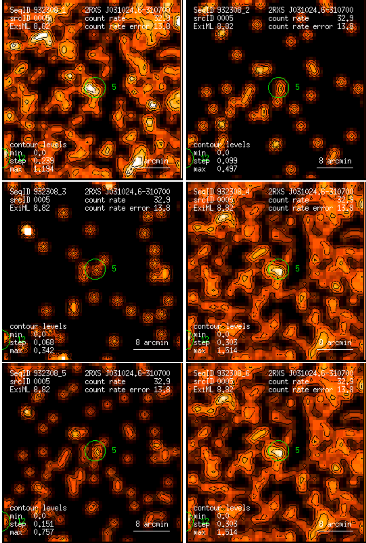
Figure 5: RASS 932308: detection 0005: band rate images, Gaussian filter: (1) PSPC channels 11 – 41, (2) 52 – 90, (3) 91 – 201, (4) 11 – 235, (5) 52 – 201, (6) 11 – 201. Broad band rates in counts/ks. Band rate contour levels in counts/ks/arcmin 2 .
