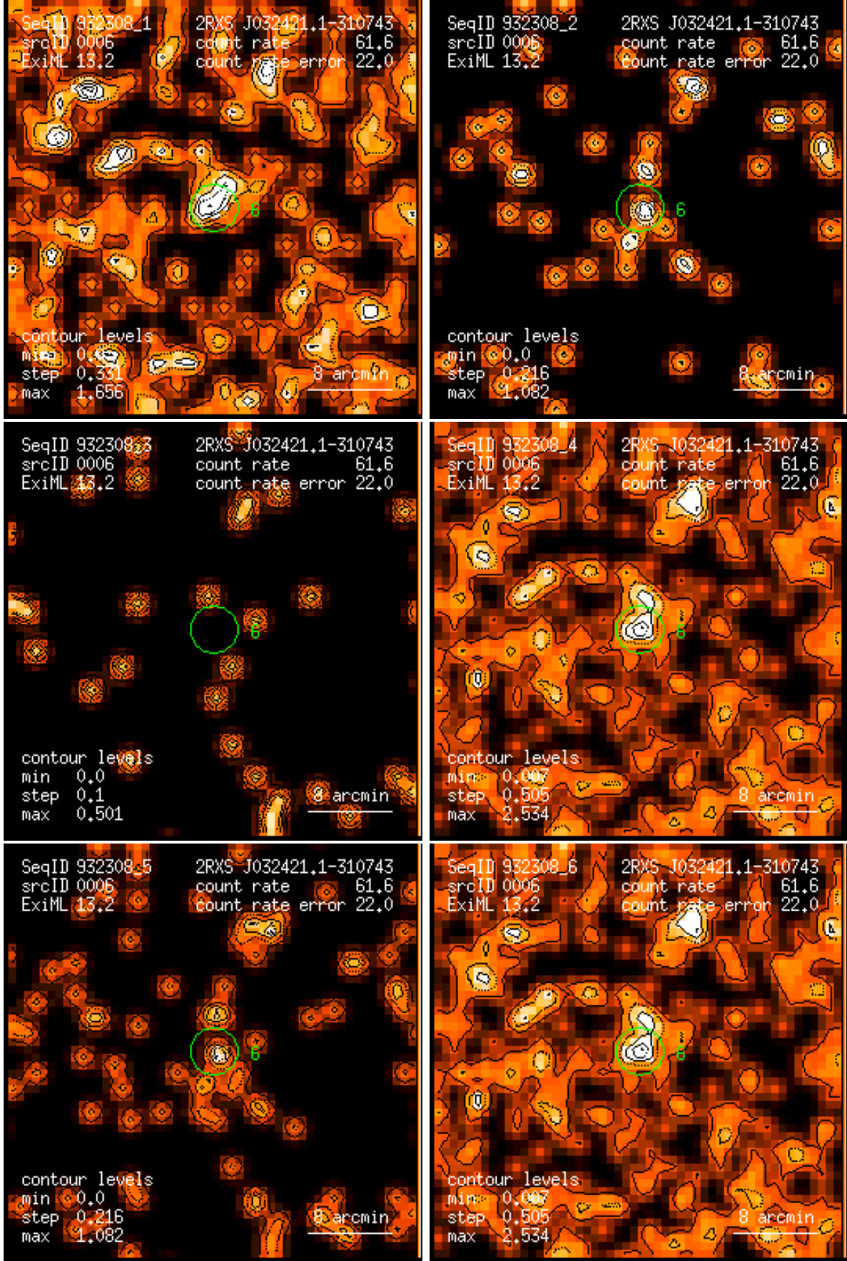
Figure 6: RASS 932308: detection 0006: band rate images, Gaussian filter: (1) PSPC channels 11 – 41, (2) 52 – 90, (3) 91 – 201, (4) 11 – 235, (5) 52 – 201, (6) 11 – 201. Broad band rates in counts/ks. Band rate contour levels in counts/ks/arcmin 2 .
