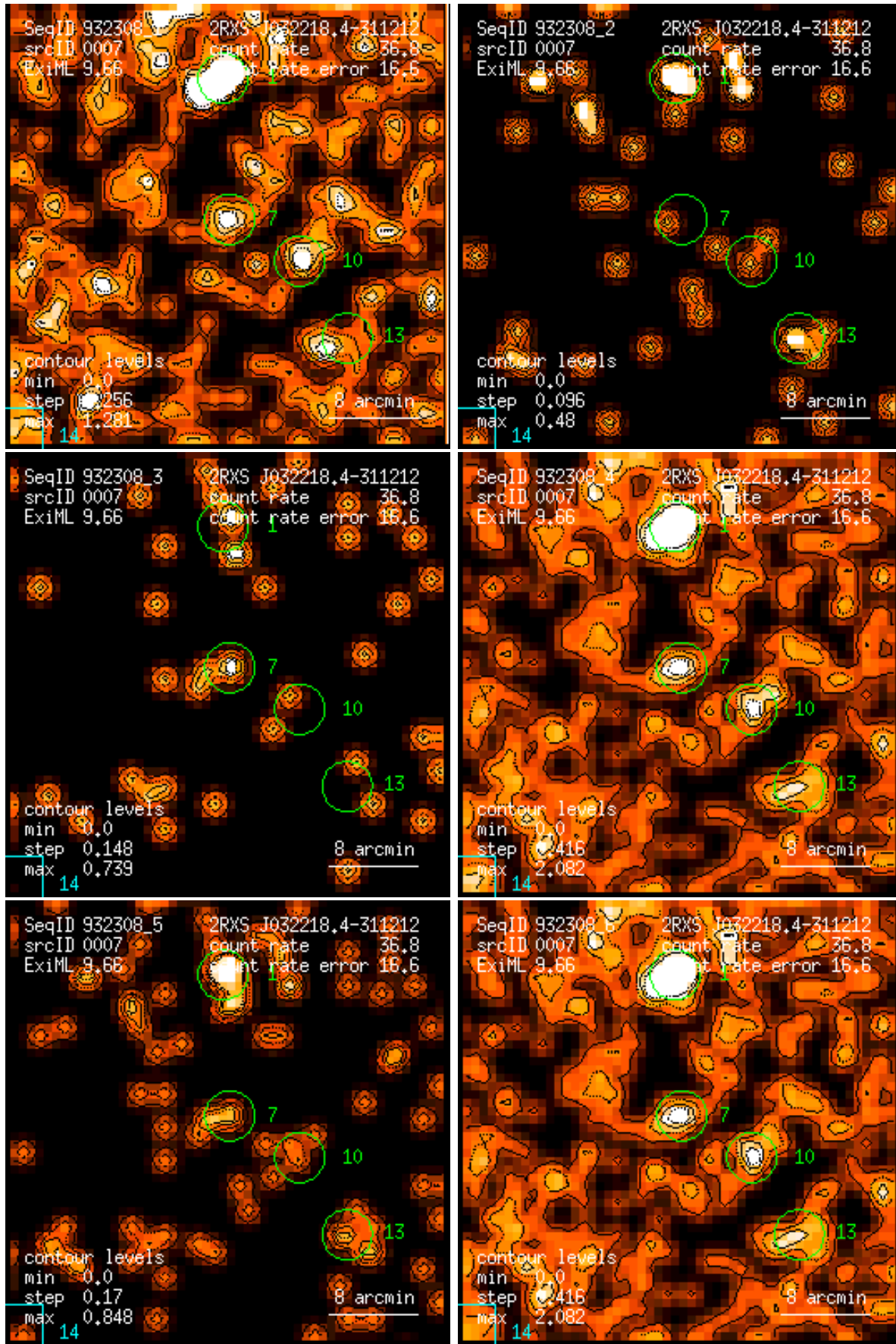
Figure 7: RASS 932308: detection 0007: band rate images, Gaussian filter: (1) PSPC channels 11 – 41, (2) 52 – 90, (3) 91 – 201, (4) 11 – 235, (5) 52 – 201, (6) 11 – 201. Broad band rates in counts/ks. Band rate contour levels in counts/ks/arcmin 2 .
