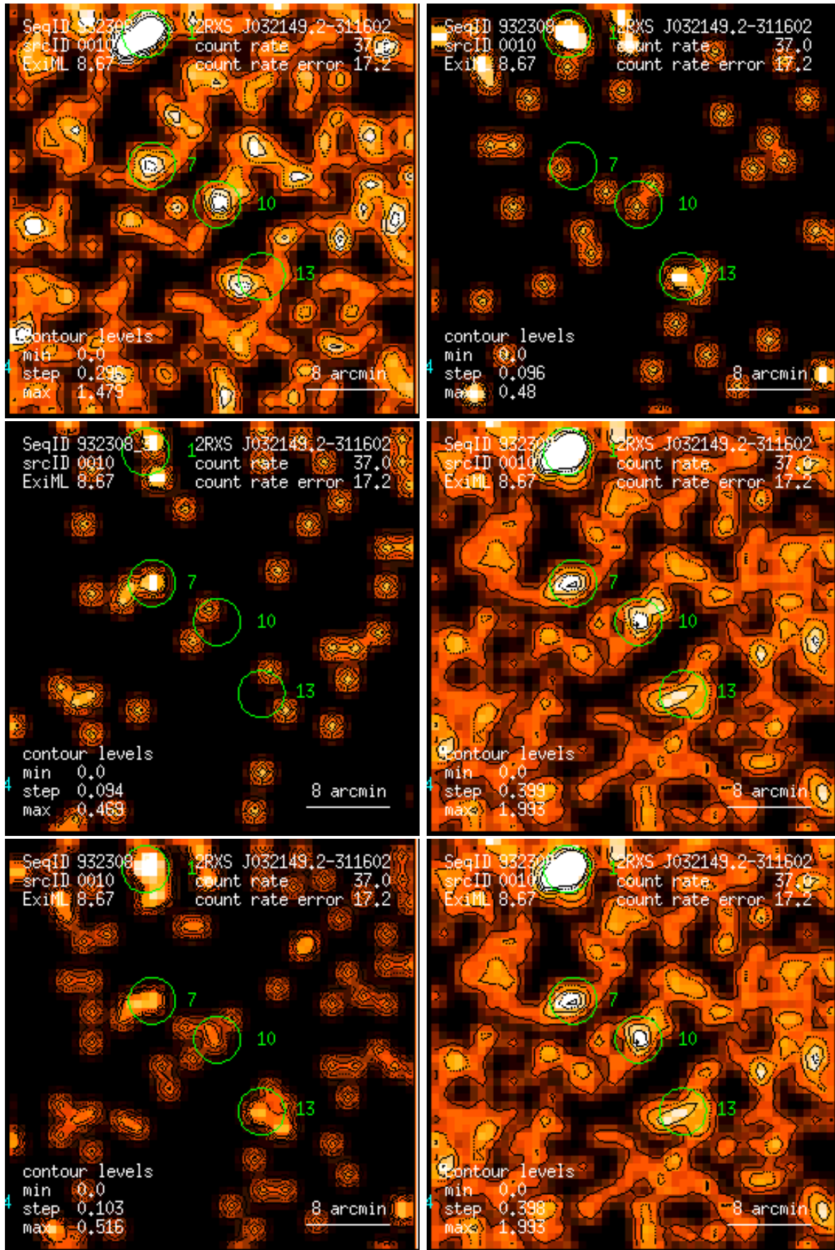
Figure 10: RASS 932308: detection 0010: band rate images, Gaussian filter: (1) PSPC channels 11 – 41, (2) 52 – 90, (3) 91 – 201, (4) 11 – 235, (5) 52 – 201, (6) 11 – 201. Broad band rates in counts/ks. Band rate contour levels in counts/ks/arcmin 2 .
