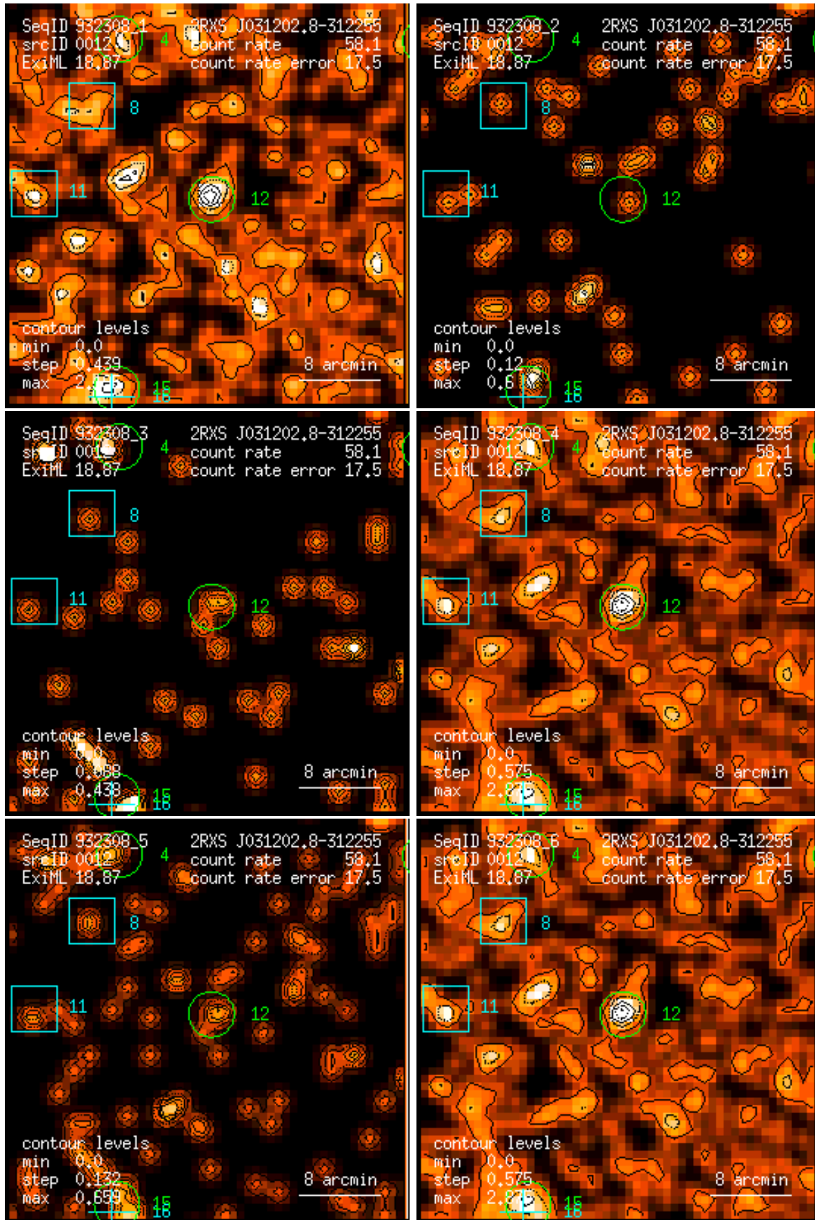
Figure 12: RASS 932308: detection 0012: band rate images, Gaussian filter: (1) PSPC channels 11 – 41, (2) 52 – 90, (3) 91 – 201, (4) 11 – 235, (5) 52 – 201, (6) 11 – 201. Broad band rates in counts/ks. Band rate contour levels in counts/ks/arcmin 2 .
