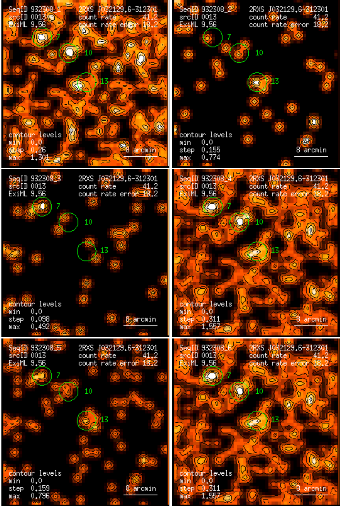
Figure 13: RASS 932308: detection 0013: band rate images, Gaussian filter: (1) PSPC channels 11 – 41, (2) 52 – 90, (3) 91 – 201, (4) 11 – 235, (5) 52 – 201, (6) 11 – 201. Broad band rates in counts/ks. Band rate contour levels in counts/ks/arcmin 2 .
