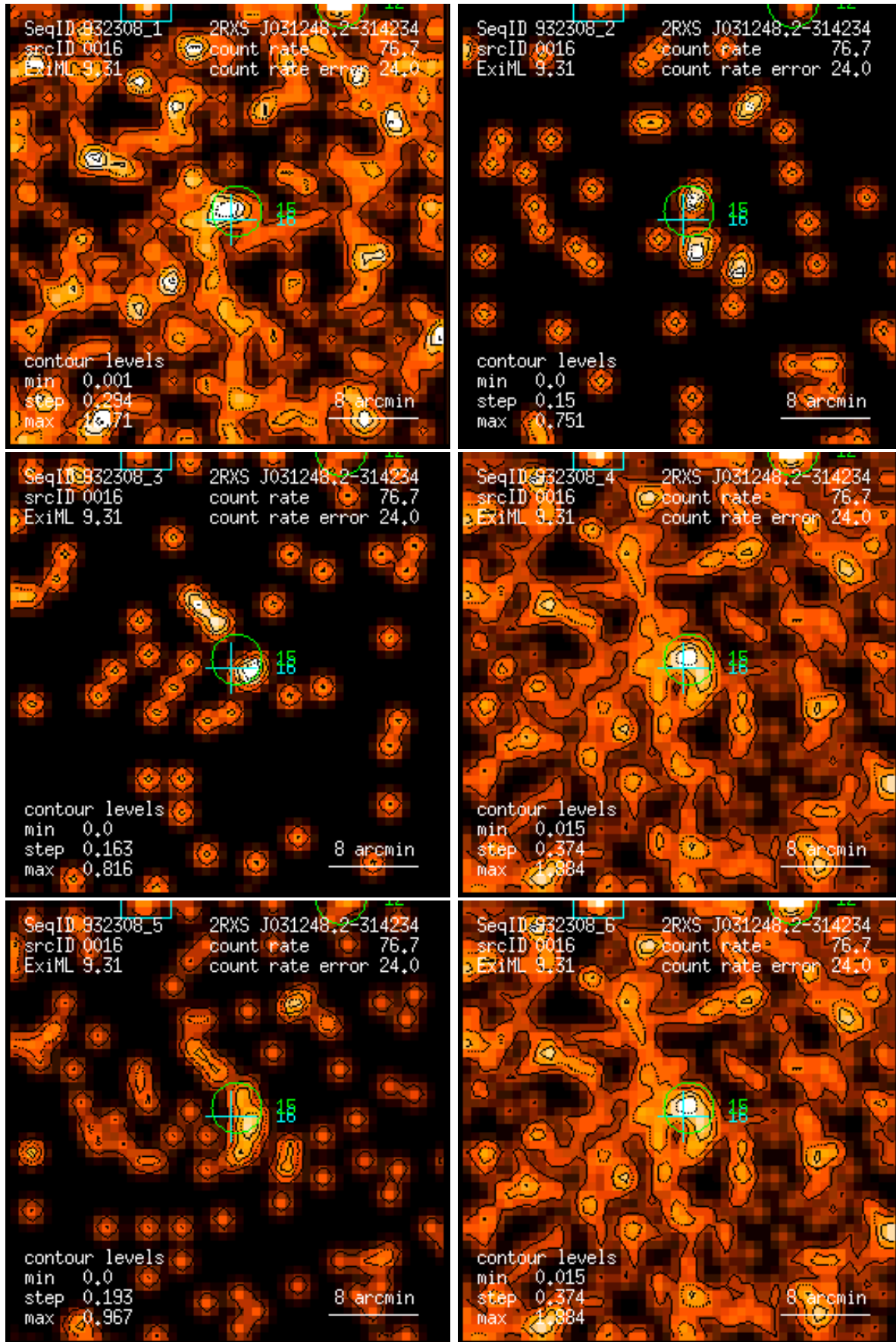
Figure 16: RASS 932308: detection 0016: band rate images, Gaussian filter: (1) PSPC channels 11 – 41, (2) 52 – 90, (3) 91 – 201, (4) 11 – 235, (5) 52 – 201, (6) 11 – 201. Broad band rates in counts/ks. Band rate contour levels in counts/ks/arcmin 2 .
