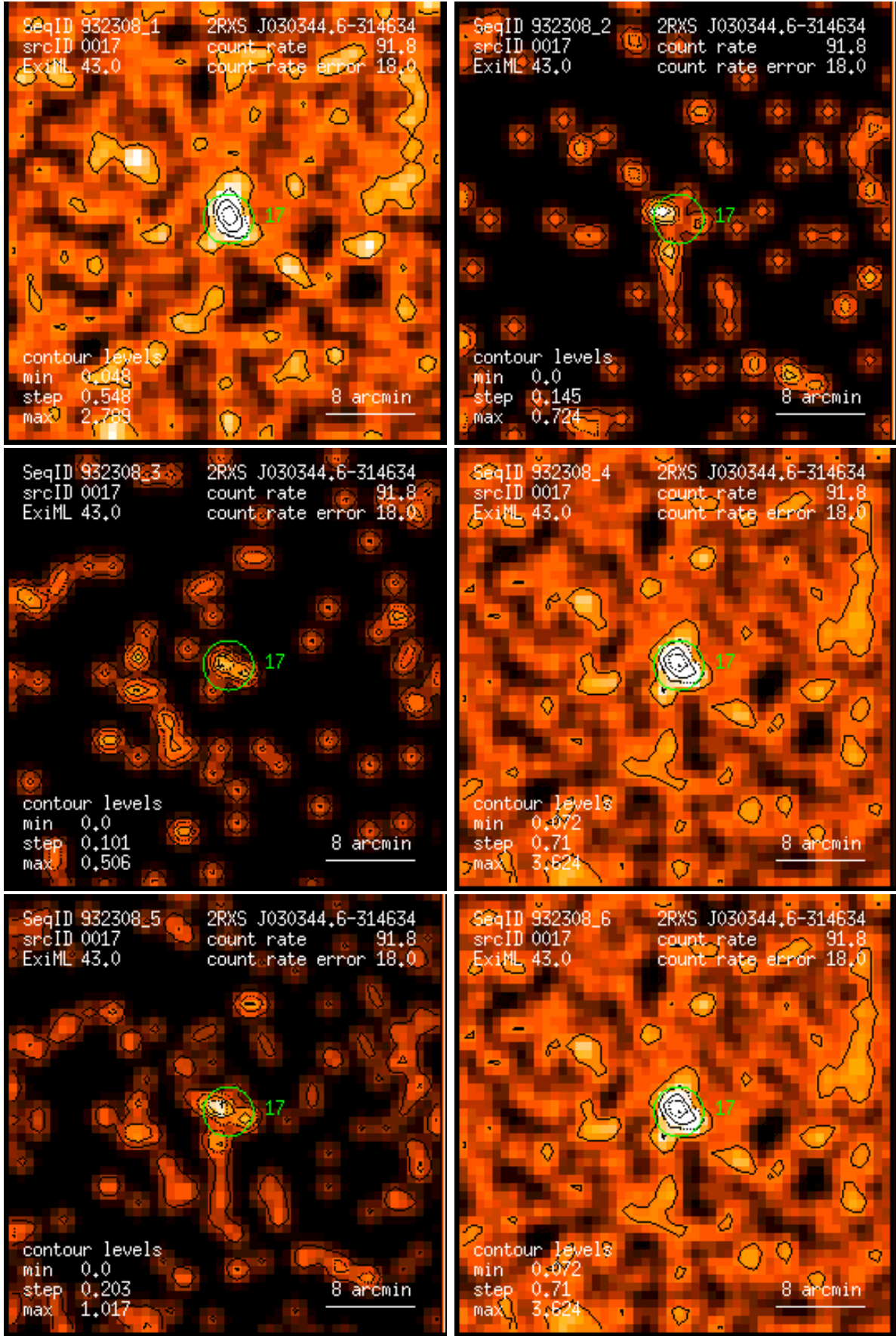
Figure 17: RASS 932308: detection 0017: band rate images, Gaussian filter: (1) PSPC channels 11 – 41, (2) 52 – 90, (3) 91 – 201, (4) 11 – 235, (5) 52 – 201, (6) 11 – 201. Broad band rates in counts/ks. Band rate contour levels in counts/ks/arcmin 2 .
