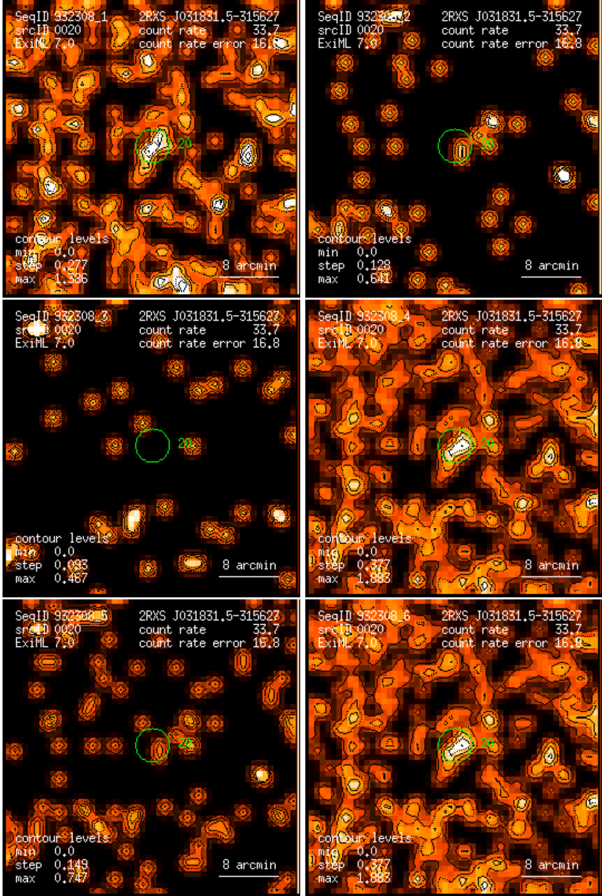
Figure 20: RASS 932308: detection 0020: band rate images, Gaussian filter: (1) PSPC channels 11 – 41, (2) 52 – 90, (3) 91 – 201, (4) 11 – 235, (5) 52 – 201, (6) 11 – 201. Broad band rates in counts/ks. Band rate contour levels in counts/ks/arcmin 2 .
