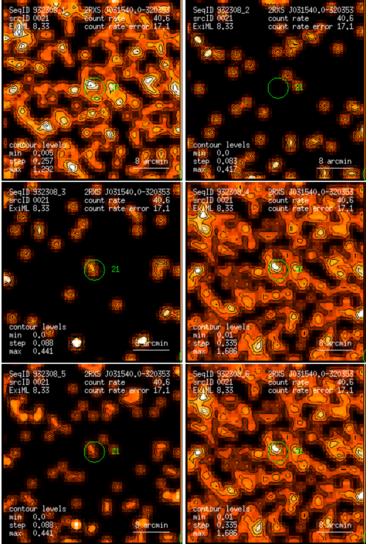
Figure 21: RASS 932308: detection 0021: band rate images, Gaussian filter: (1) PSPC channels 11 – 41, (2) 52 – 90, (3) 91 – 201, (4) 11 – 235, (5) 52 – 201, (6) 11 – 201. Broad band rates in counts/ks. Band rate contour levels in counts/ks/arcmin 2 .
