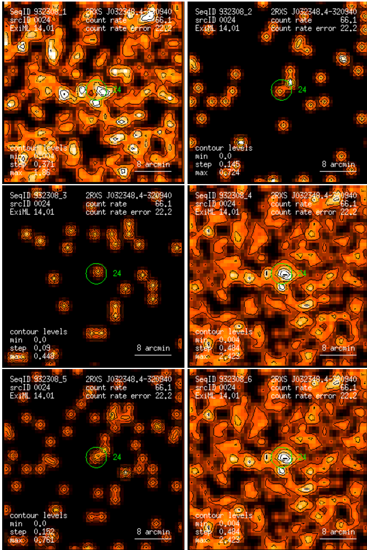
Figure 24: RASS 932308: detection 0024: band rate images, Gaussian filter: (1) PSPC channels 11 – 41, (2) 52 – 90, (3) 91 – 201, (4) 11 – 235, (5) 52 – 201, (6) 11 – 201. Broad band rates in counts/ks. Band rate contour levels in counts/ks/arcmin 2 .
