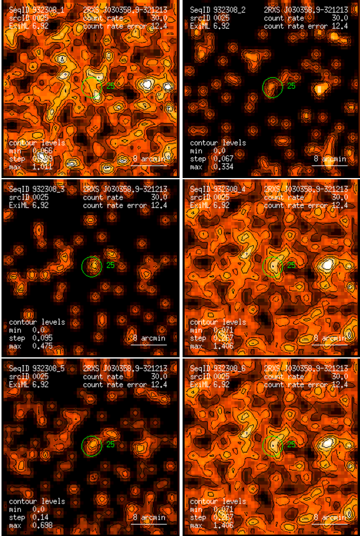
Figure 25: RASS 932308: detection 0025: band rate images, Gaussian filter: (1) PSPC channels 11 – 41, (2) 52 – 90, (3) 91 – 201, (4) 11 – 235, (5) 52 – 201, (6) 11 – 201. Broad band rates in counts/ks. Band rate contour levels in counts/ks/arcmin 2 .
