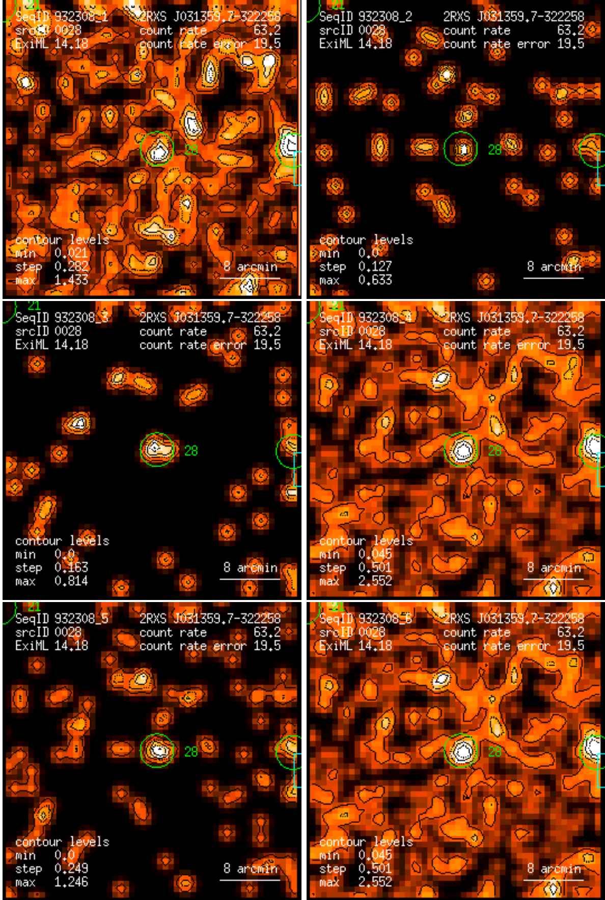
Figure 28: RASS 932308: detection 0028: band rate images, Gaussian filter: (1) PSPC channels 11 – 41, (2) 52 – 90, (3) 91 – 201, (4) 11 – 235, (5) 52 – 201, (6) 11 – 201. Broad band rates in counts/ks. Band rate contour levels in counts/ks/arcmin 2 .
