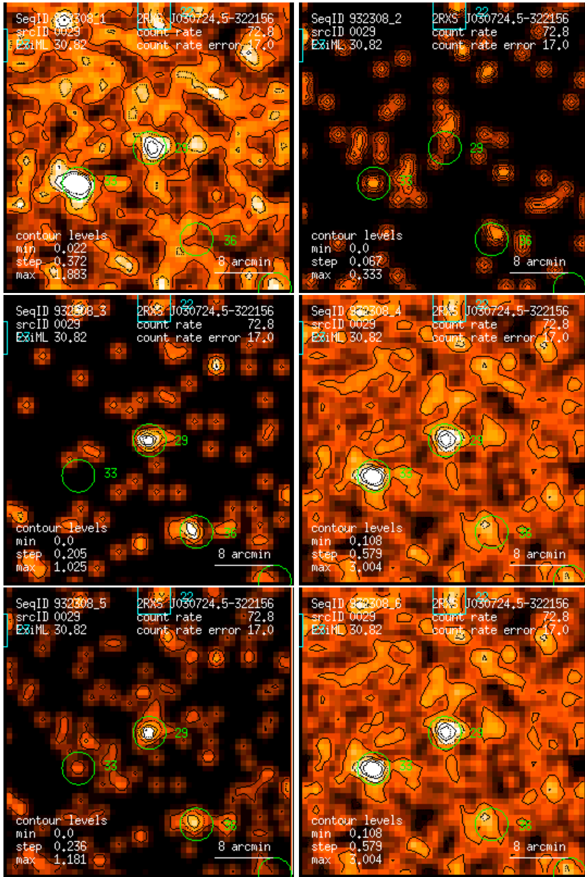
Figure 29: RASS 932308: detection 0029: band rate images, Gaussian filter: (1) PSPC channels 11 – 41, (2) 52 – 90, (3) 91 – 201, (4) 11 – 235, (5) 52 – 201, (6) 11 – 201. Broad band rates in counts/ks. Band rate contour levels in counts/ks/arcmin 2 .
