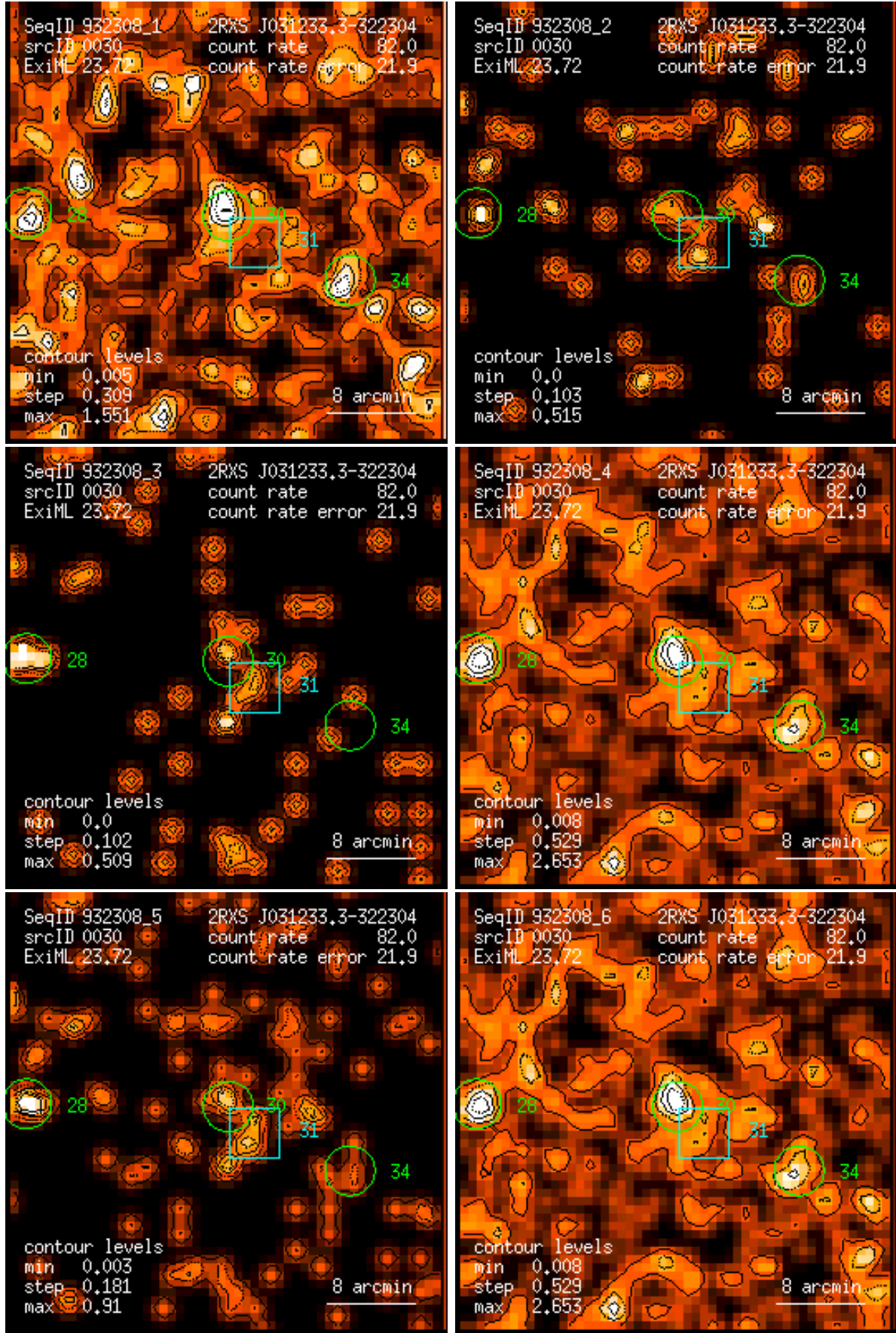
Figure 30: RASS 932308: detection 0030: band rate images, Gaussian filter: (1) PSPC channels 11 – 41, (2) 52 – 90, (3) 91 – 201, (4) 11 – 235, (5) 52 – 201, (6) 11 – 201. Broad band rates in counts/ks. Band rate contour levels in counts/ks/arcmin 2 .
