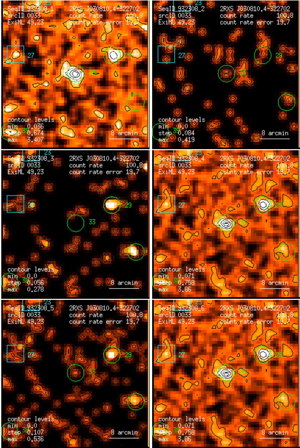
Figure 33: RASS 932308: detection 0033: band rate images, Gaussian filter: (1) PSPC channels 11 – 41, (2) 52 – 90, (3) 91 – 201, (4) 11 – 235, (5) 52 – 201, (6) 11 – 201. Broad band rates in counts/ks. Band rate contour levels in counts/ks/arcmin 2 .
