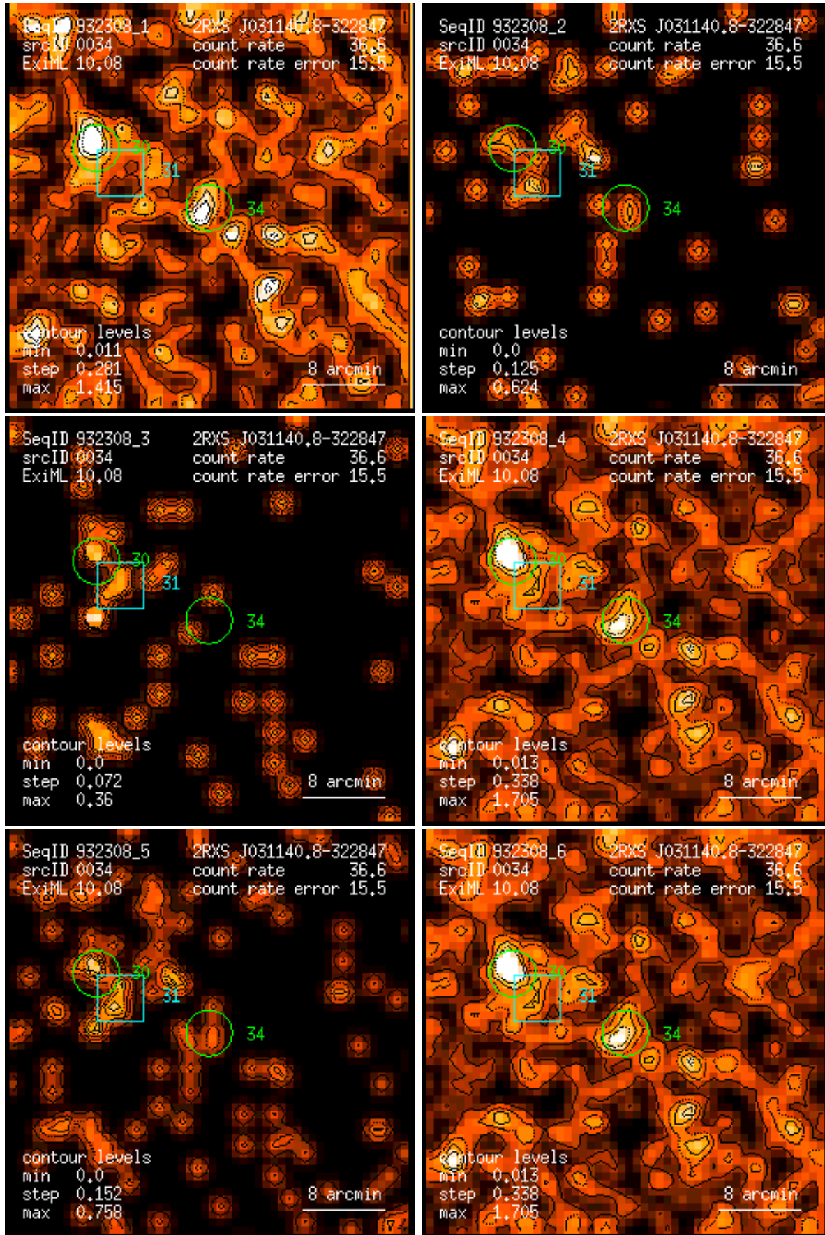
Figure 34: RASS 932308: detection 0034: band rate images, Gaussian filter: (1) PSPC channels 11 – 41, (2) 52 – 90, (3) 91 – 201, (4) 11 – 235, (5) 52 – 201, (6) 11 – 201. Broad band rates in counts/ks. Band rate contour levels in counts/ks/arcmin 2 .
