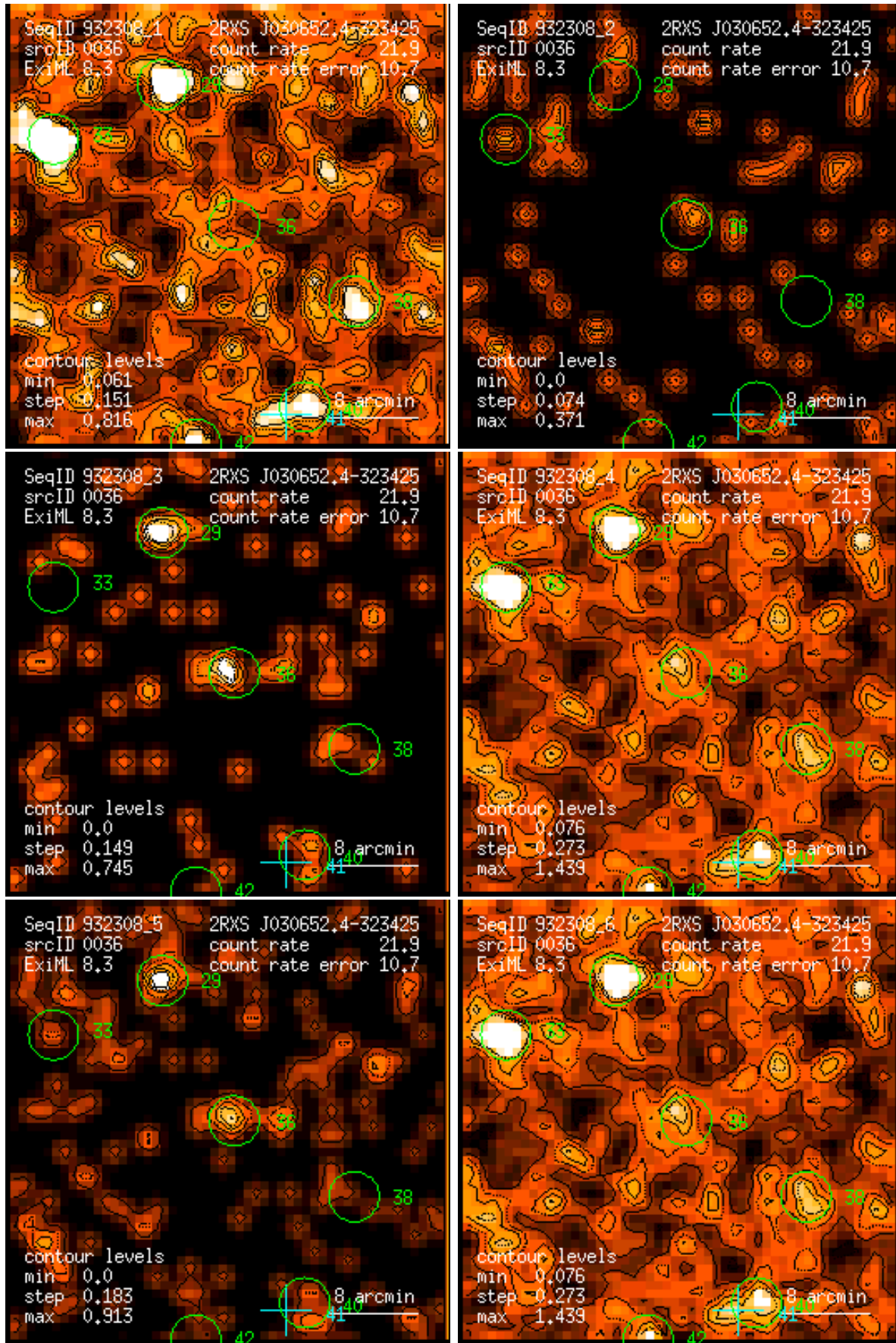
Figure 36: RASS 932308: detection 0036: band rate images, Gaussian filter: (1) PSPC channels 11 – 41, (2) 52 – 90, (3) 91 – 201, (4) 11 – 235, (5) 52 – 201, (6) 11 – 201. Broad band rates in counts/ks. Band rate contour levels in counts/ks/arcmin 2 .
