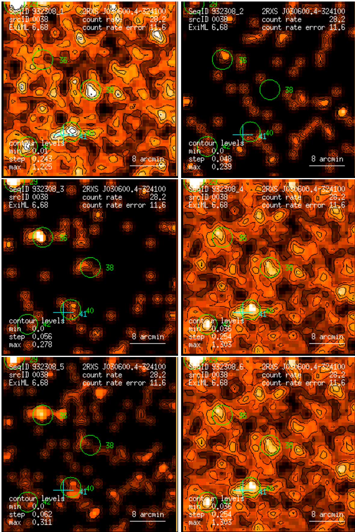
Figure 38: RASS 932308: detection 0038: band rate images, Gaussian filter: (1) PSPC channels 11 – 41, (2) 52 – 90, (3) 91 – 201, (4) 11 – 235, (5) 52 – 201, (6) 11 – 201. Broad band rates in counts/ks. Band rate contour levels in counts/ks/arcmin 2 .
