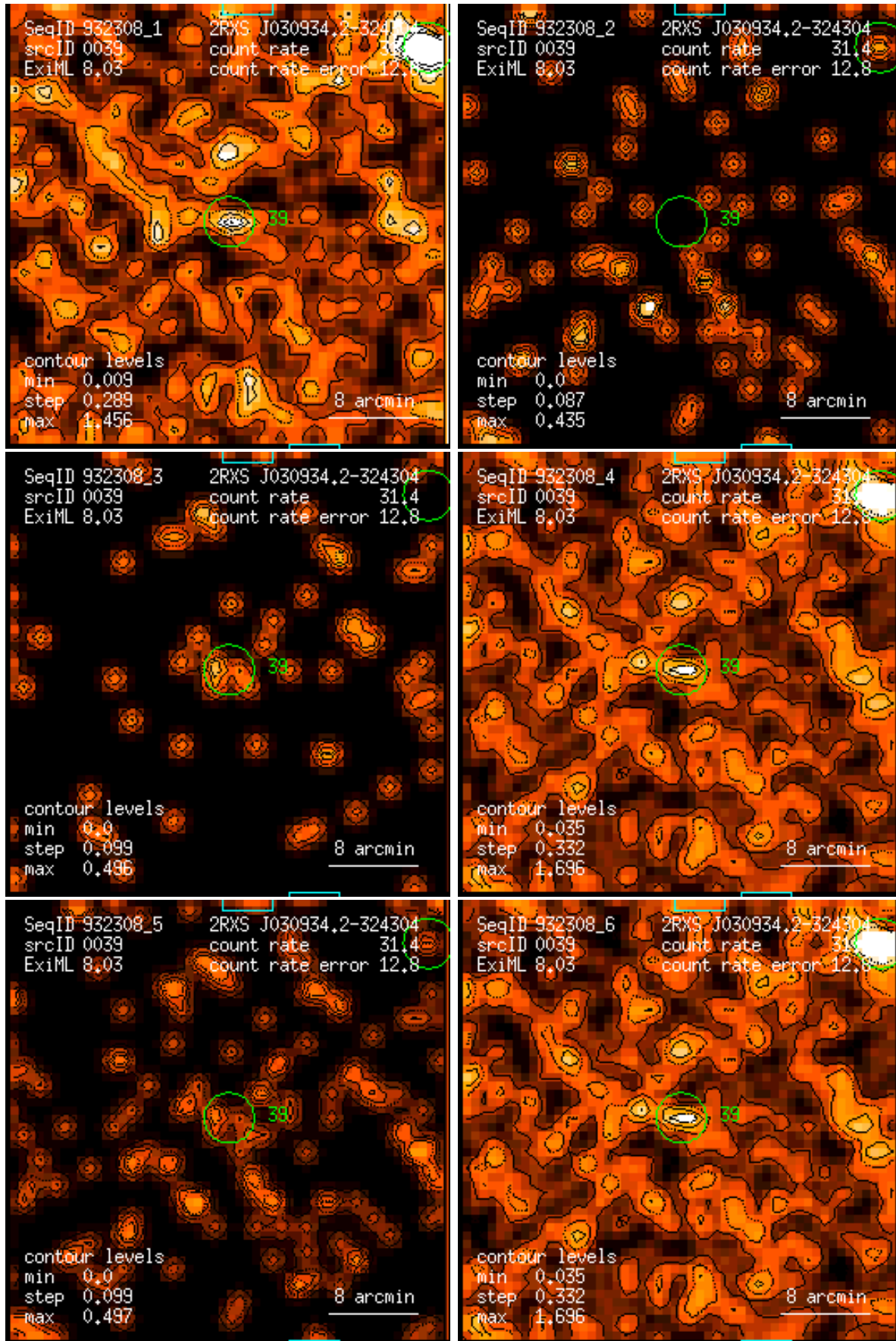
Figure 39: RASS 932308: detection 0039: band rate images, Gaussian filter: (1) PSPC channels 11 – 41, (2) 52 – 90, (3) 91 – 201, (4) 11 – 235, (5) 52 – 201, (6) 11 – 201. Broad band rates in counts/ks. Band rate contour levels in counts/ks/arcmin 2 .
