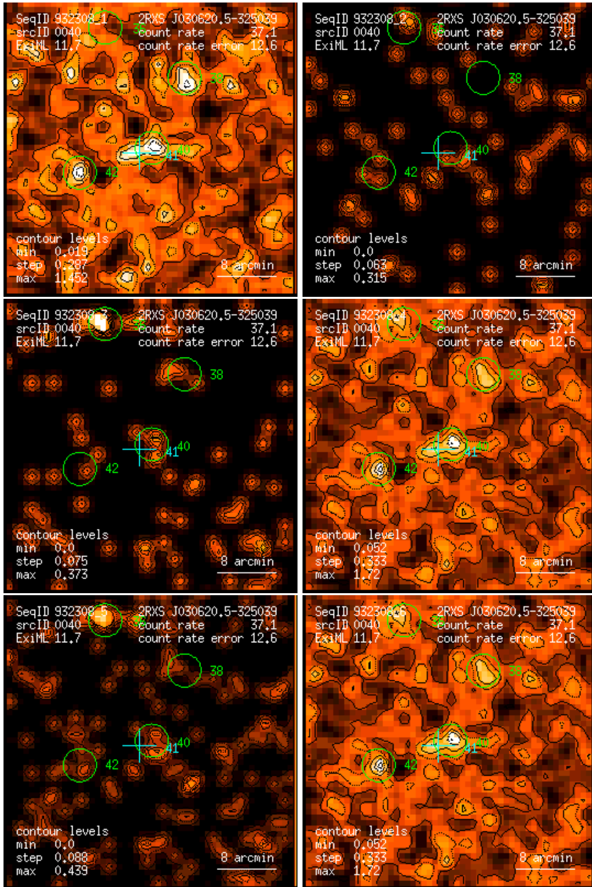
Figure 40: RASS 932308: detection 0040: band rate images, Gaussian filter: (1) PSPC channels 11 – 41, (2) 52 – 90, (3) 91 – 201, (4) 11 – 235, (5) 52 – 201, (6) 11 – 201. Broad band rates in counts/ks. Band rate contour levels in counts/ks/arcmin 2 .
