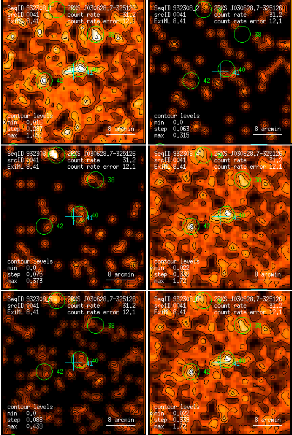
Figure 41: RASS 932308: detection 0041: band rate images, Gaussian filter: (1) PSPC channels 11 – 41, (2) 52 – 90, (3) 91 – 201, (4) 11 – 235, (5) 52 – 201, (6) 11 – 201. Broad band rates in counts/ks. Band rate contour levels in counts/ks/arcmin 2 .
