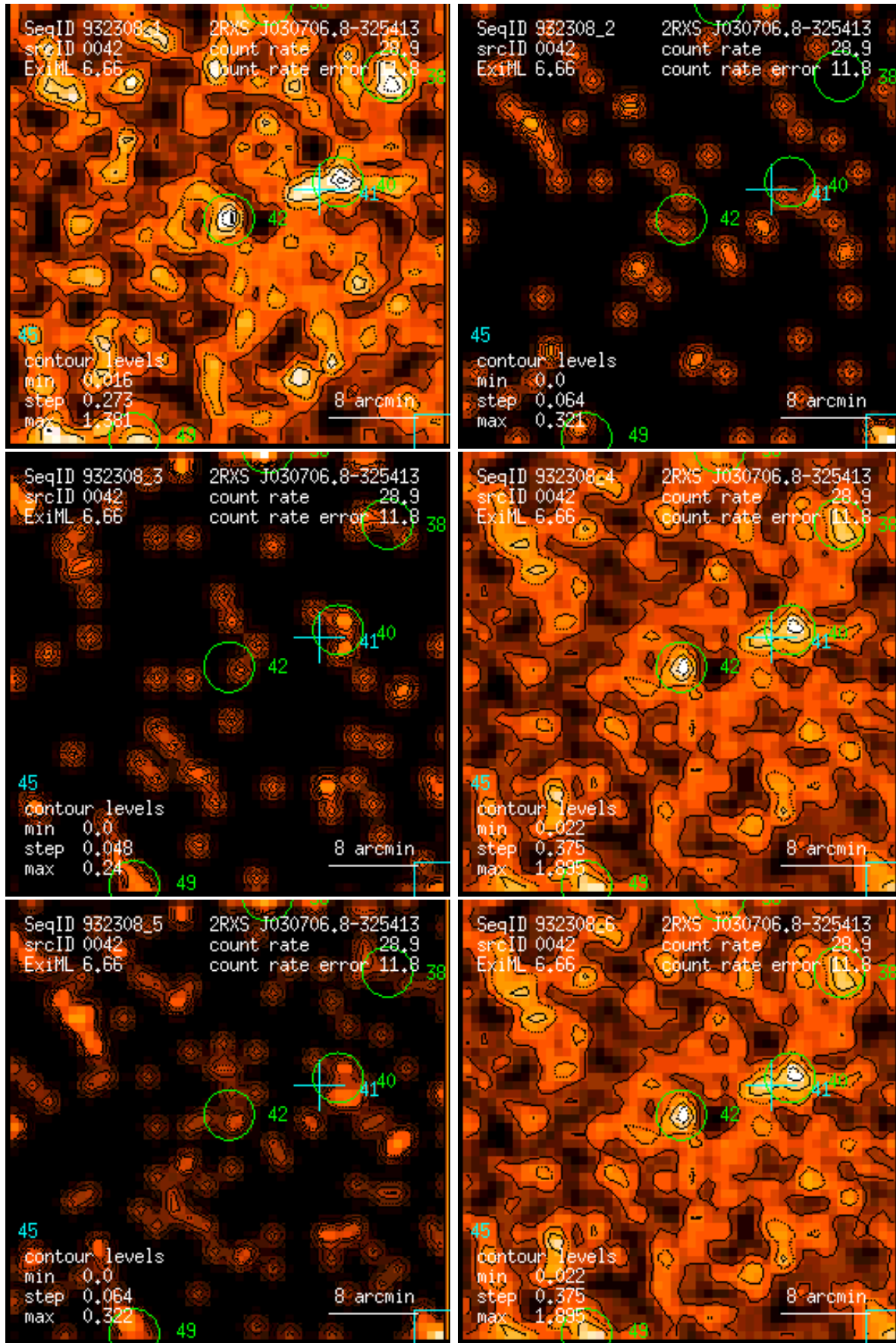
Figure 42: RASS 932308: detection 0042: band rate images, Gaussian filter: (1) PSPC channels 11 – 41, (2) 52 – 90, (3) 91 – 201, (4) 11 – 235, (5) 52 – 201, (6) 11 – 201. Broad band rates in counts/ks. Band rate contour levels in counts/ks/arcmin 2 .
