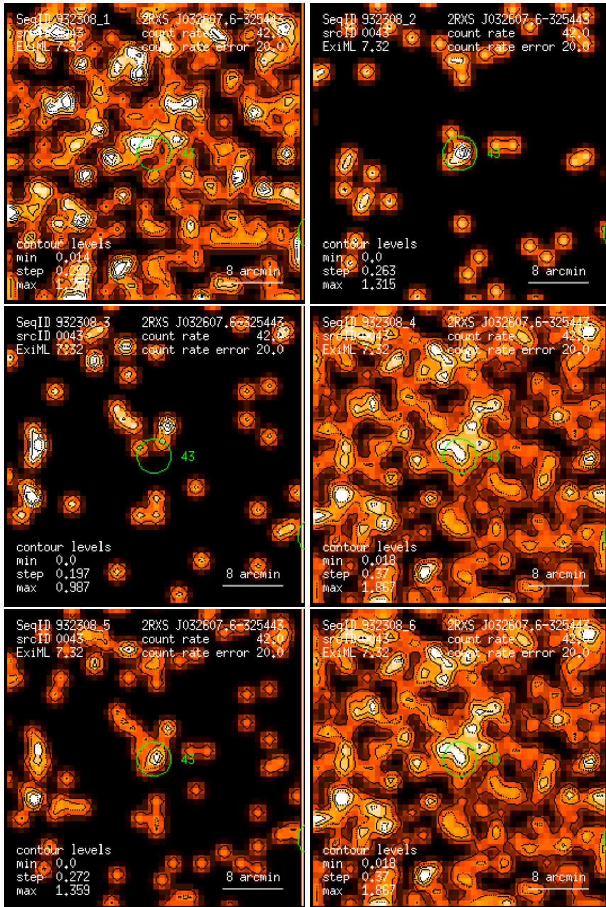
Figure 43: RASS 932308: detection 0043: band rate images, Gaussian filter: (1) PSPC channels 11 – 41, (2) 52 – 90, (3) 91 – 201, (4) 11 – 235, (5) 52 – 201, (6) 11 – 201. Broad band rates in counts/ks. Band rate contour levels in counts/ks/arcmin 2 .
