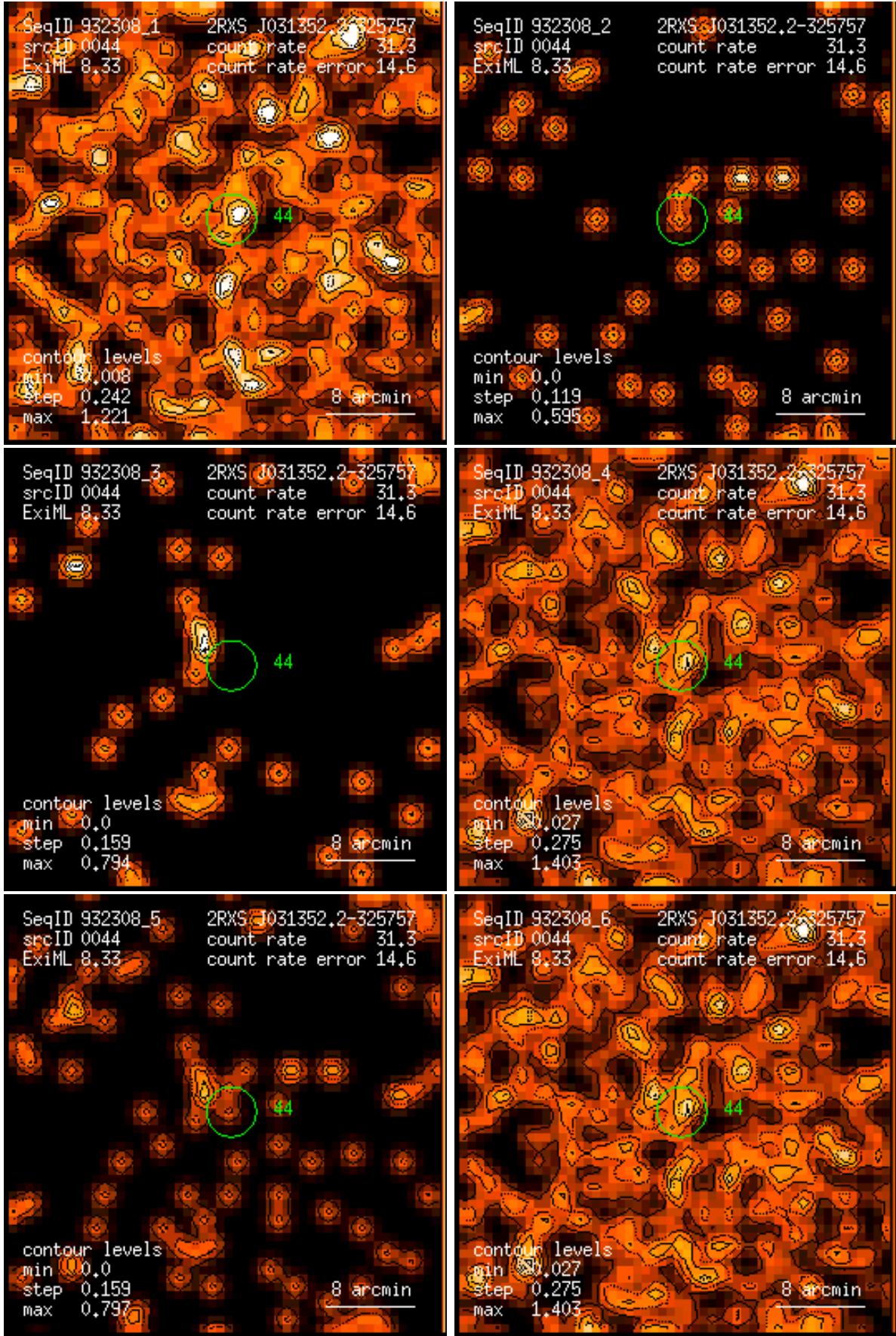
Figure 44: RASS 932308: detection 0044: band rate images, Gaussian filter: (1) PSPC channels 11 – 41, (2) 52 – 90, (3) 91 – 201, (4) 11 – 235, (5) 52 – 201, (6) 11 – 201. Broad band rates in counts/ks. Band rate contour levels in counts/ks/arcmin 2 .
