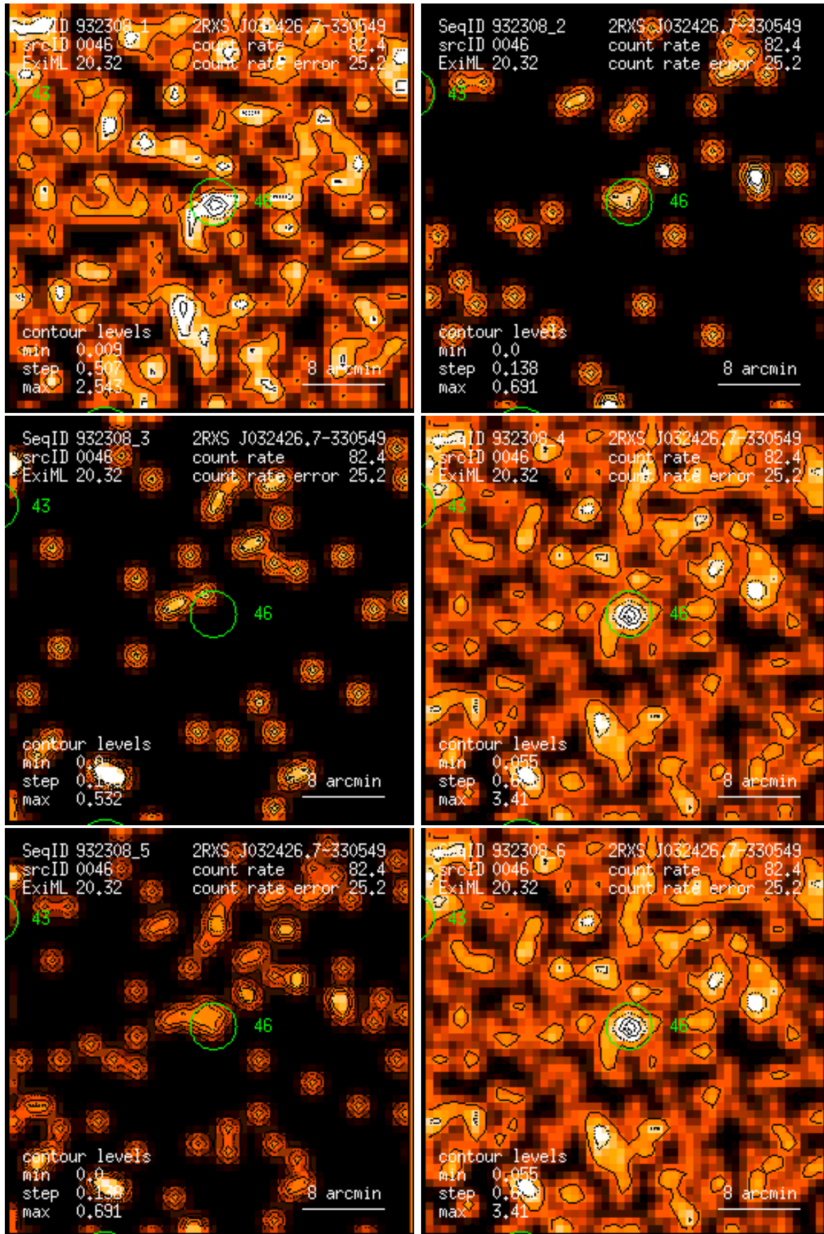
Figure 46: RASS 932308: detection 0046: band rate images, Gaussian filter: (1) PSPC channels 11 – 41, (2) 52 – 90, (3) 91 – 201, (4) 11 – 235, (5) 52 – 201, (6) 11 – 201. Broad band rates in counts/ks. Band rate contour levels in counts/ks/arcmin 2 .
