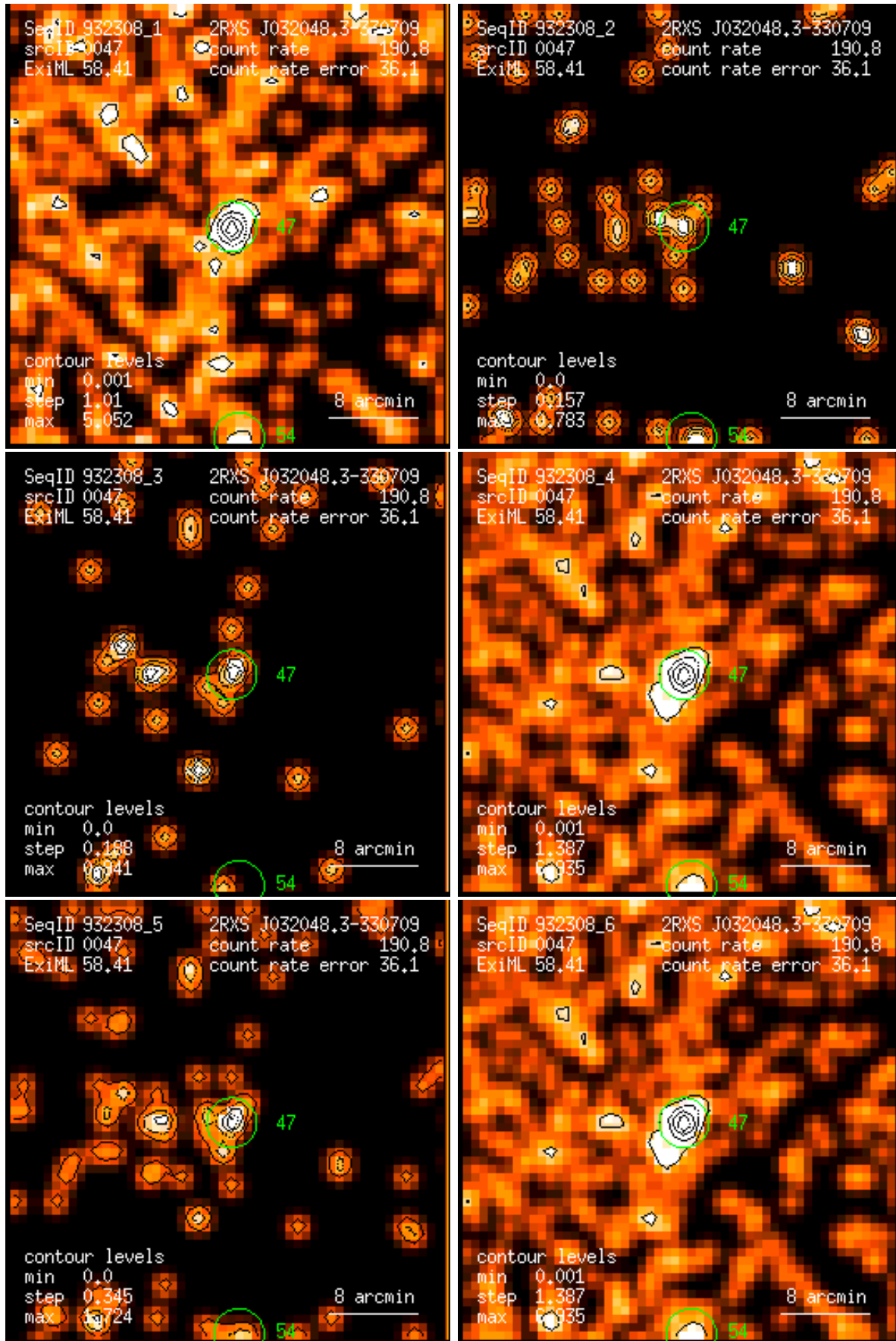
Figure 47: RASS 932308: detection 0047: band rate images, Gaussian filter: (1) PSPC channels 11 – 41, (2) 52 – 90, (3) 91 – 201, (4) 11 – 235, (5) 52 – 201, (6) 11 – 201. Broad band rates in counts/ks. Band rate contour levels in counts/ks/arcmin 2 .
