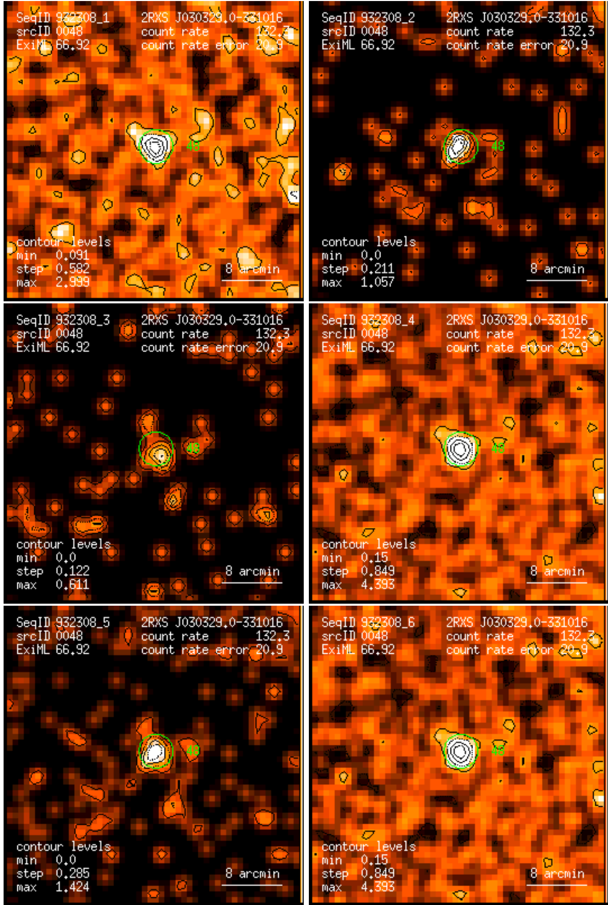
Figure 48: RASS 932308: detection 0048: band rate images, Gaussian filter: (1) PSPC channels 11 – 41, (2) 52 – 90, (3) 91 – 201, (4) 11 – 235, (5) 52 – 201, (6) 11 – 201. Broad band rates in counts/ks. Band rate contour levels in counts/ks/arcmin 2 .
