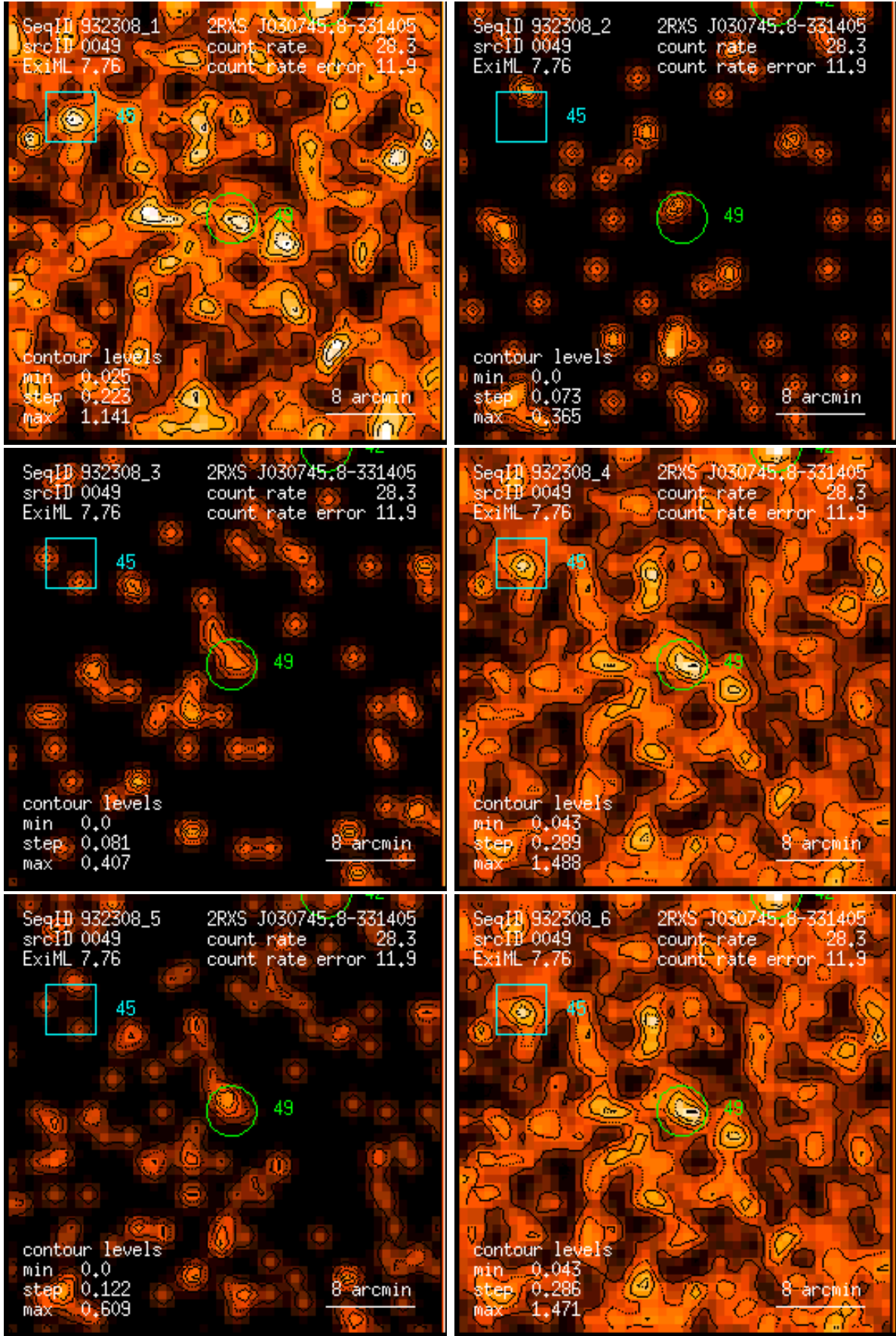
Figure 49: RASS 932308: detection 0049: band rate images, Gaussian filter: (1) PSPC channels 11 – 41, (2) 52 – 90, (3) 91 – 201, (4) 11 – 235, (5) 52 – 201, (6) 11 – 201. Broad band rates in counts/ks. Band rate contour levels in counts/ks/arcmin 2 .
