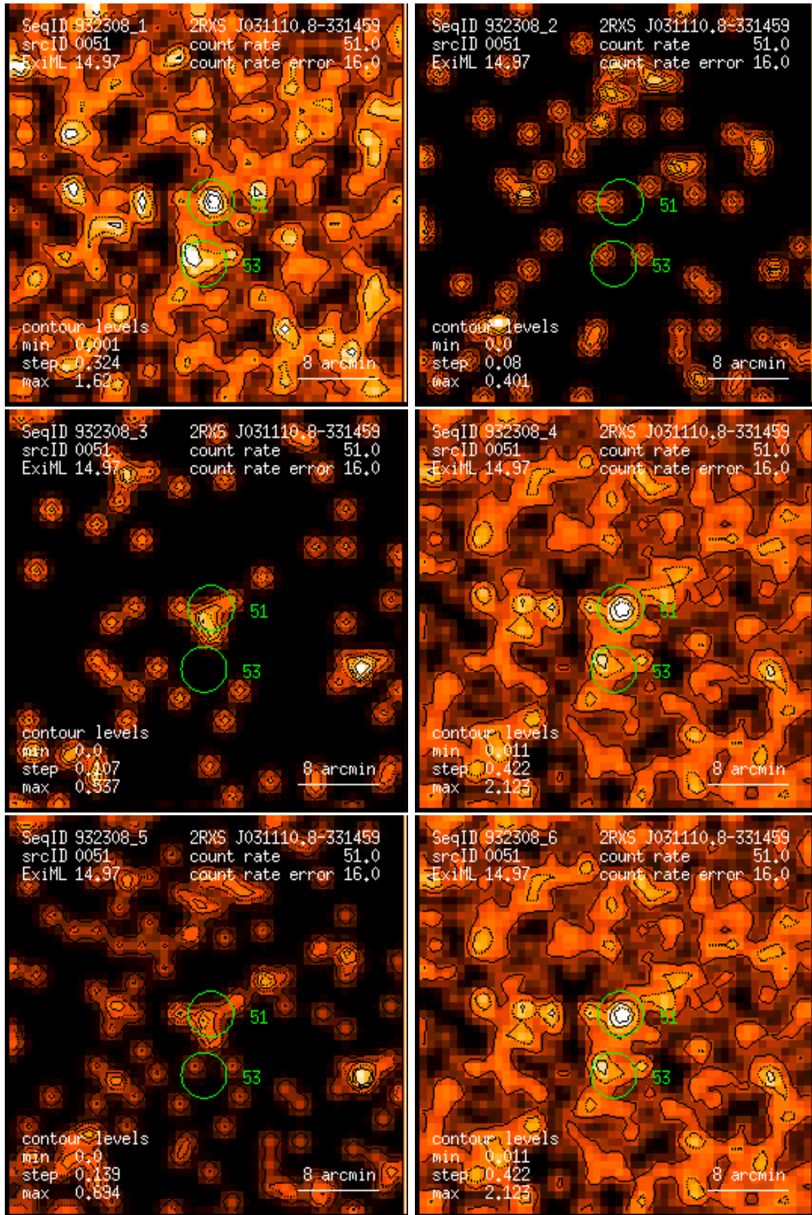
Figure 51: RASS 932308: detection 0051: band rate images, Gaussian filter: (1) PSPC channels 11 – 41, (2) 52 – 90, (3) 91 – 201, (4) 11 – 235, (5) 52 – 201, (6) 11 – 201. Broad band rates in counts/ks. Band rate contour levels in counts/ks/arcmin 2 .
