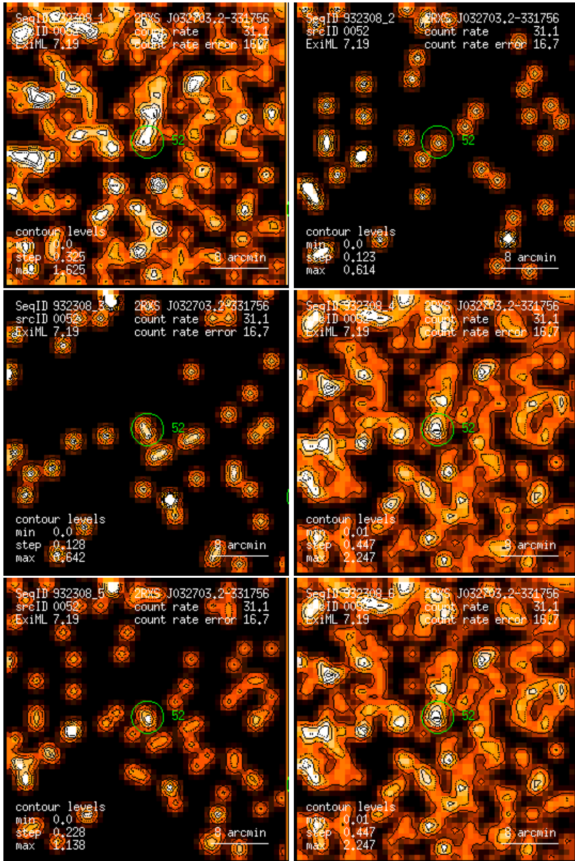
Figure 52: RASS 932308: detection 0052: band rate images, Gaussian filter: (1) PSPC channels 11 – 41, (2) 52 – 90, (3) 91 – 201, (4) 11 – 235, (5) 52 – 201, (6) 11 – 201. Broad band rates in counts/ks. Band rate contour levels in counts/ks/arcmin 2 .
