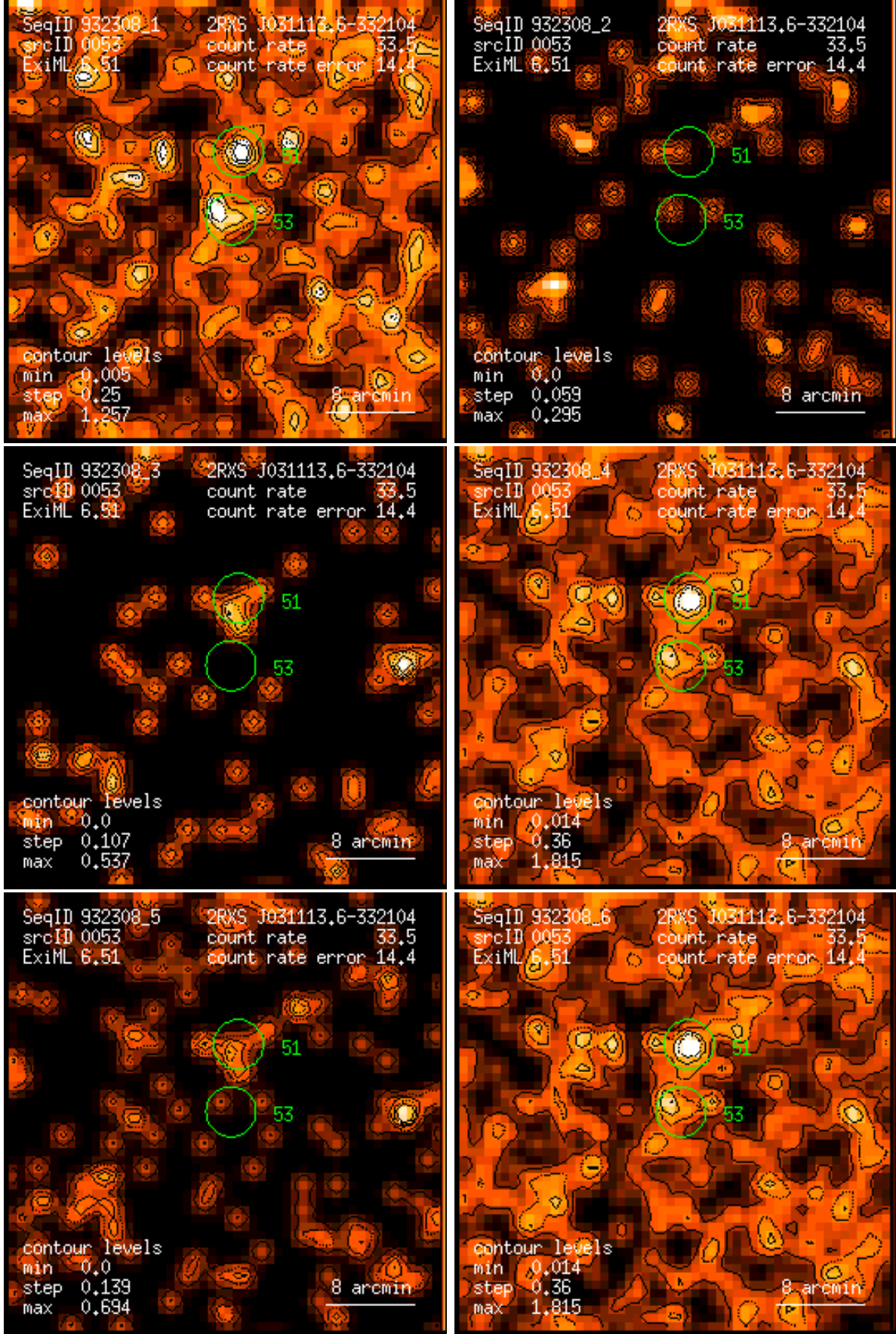
Figure 53: RASS 932308: detection 0053: band rate images, Gaussian filter: (1) PSPC channels 11 – 41, (2) 52 – 90, (3) 91 – 201, (4) 11 – 235, (5) 52 – 201, (6) 11 – 201. Broad band rates in counts/ks. Band rate contour levels in counts/ks/arcmin 2 .
