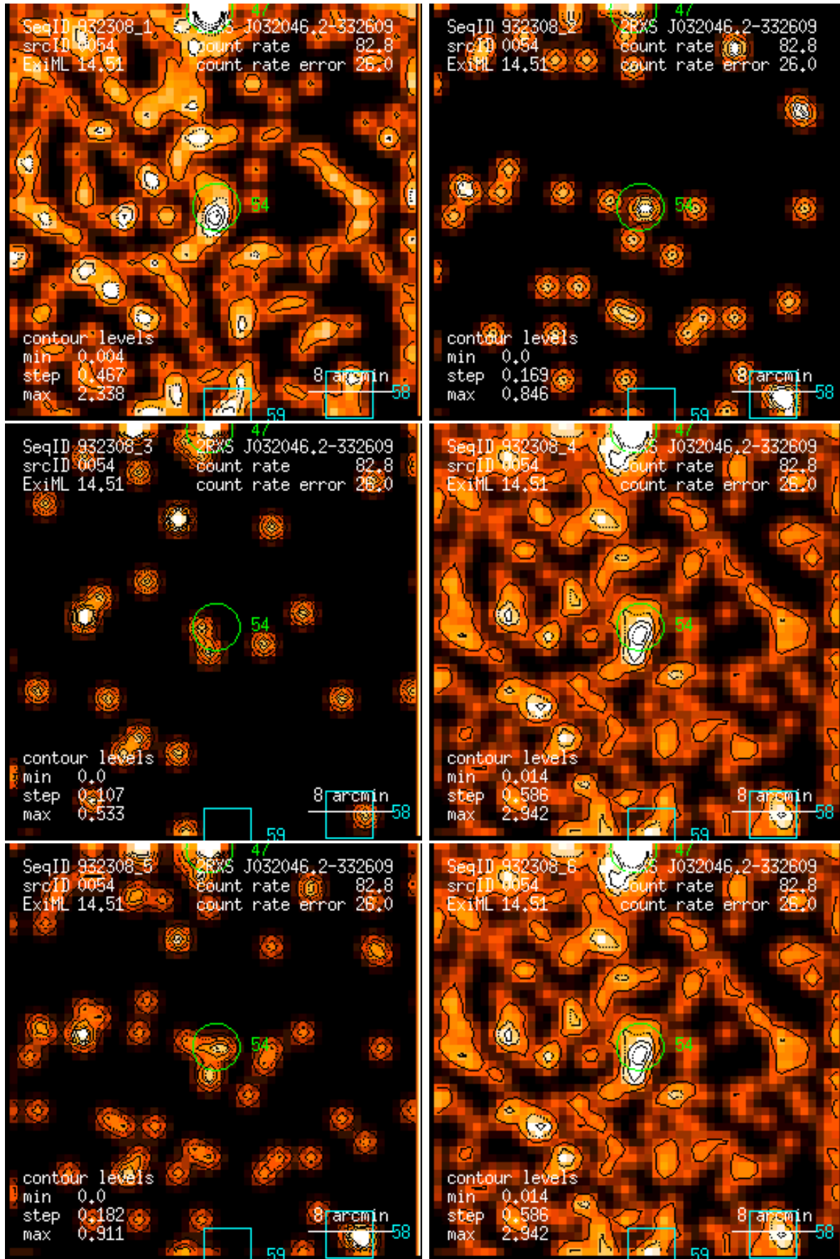
Figure 54: RASS 932308: detection 0054: band rate images, Gaussian filter: (1) PSPC channels 11 – 41, (2) 52 – 90, (3) 91 – 201, (4) 11 – 235, (5) 52 – 201, (6) 11 – 201. Broad band rates in counts/ks. Band rate contour levels in counts/ks/arcmin 2 .
