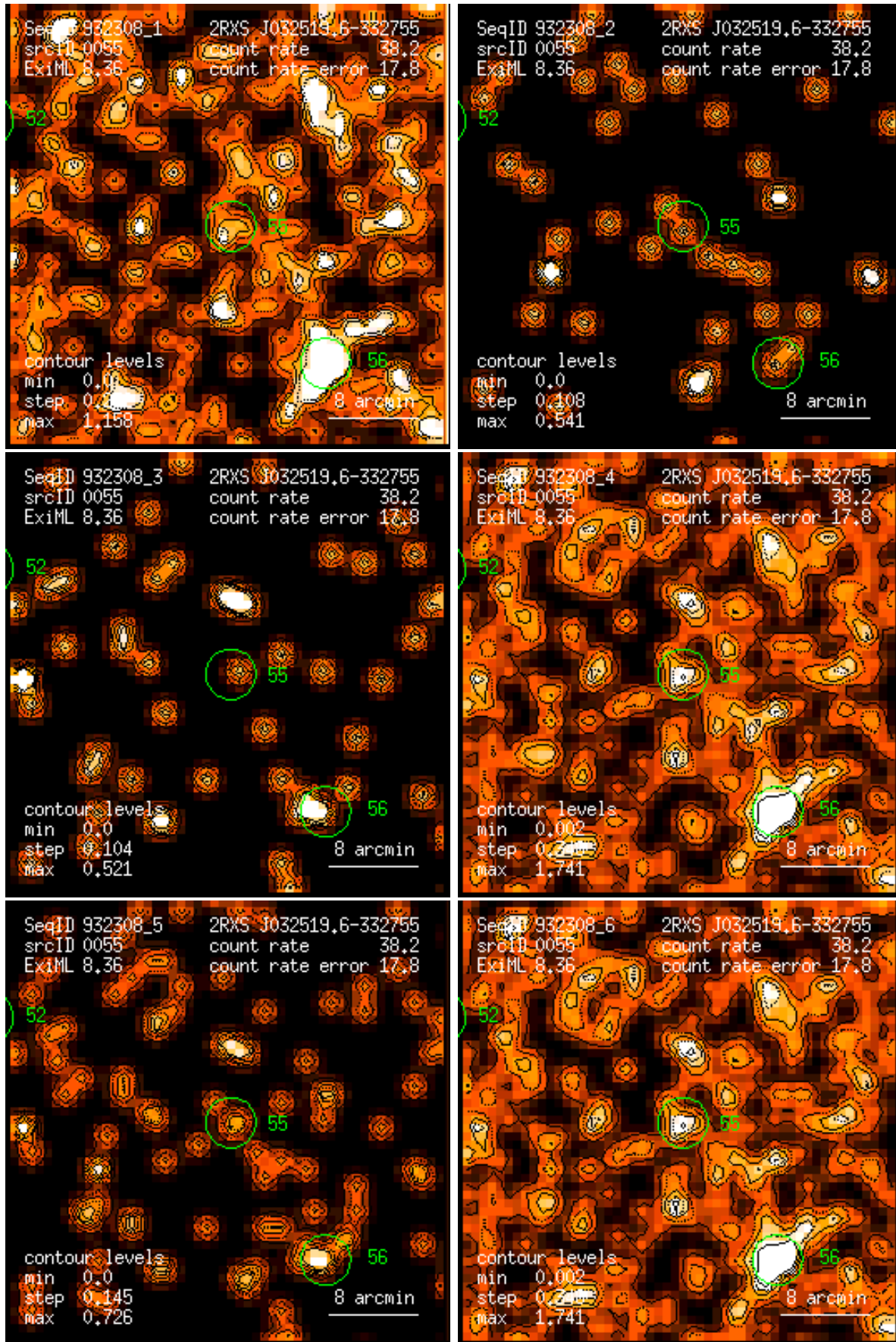
Figure 55: RASS 932308: detection 0055: band rate images, Gaussian filter: (1) PSPC channels 11 – 41, (2) 52 – 90, (3) 91 – 201, (4) 11 – 235, (5) 52 – 201, (6) 11 – 201. Broad band rates in counts/ks. Band rate contour levels in counts/ks/arcmin 2 .
