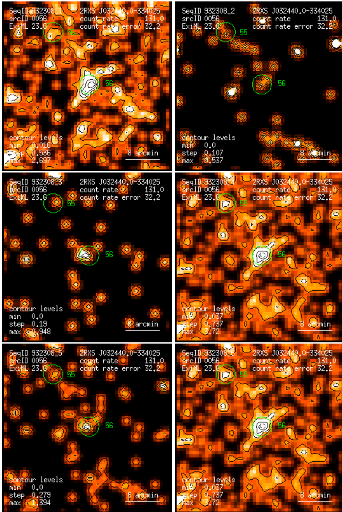
Figure 56: RASS 932308: detection 0056: band rate images, Gaussian filter: (1) PSPC channels 11 – 41, (2) 52 – 90, (3) 91 – 201, (4) 11 – 235, (5) 52 – 201, (6) 11 – 201. Broad band rates in counts/ks. Band rate contour levels in counts/ks/arcmin 2 .
