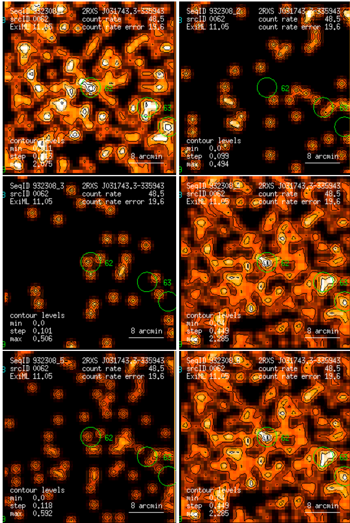
Figure 62: RASS 932308: detection 0062: band rate images, Gaussian filter: (1) PSPC channels 11 – 41, (2) 52 – 90, (3) 91 – 201, (4) 11 – 235, (5) 52 – 201, (6) 11 – 201. Broad band rates in counts/ks. Band rate contour levels in counts/ks/arcmin 2 .
