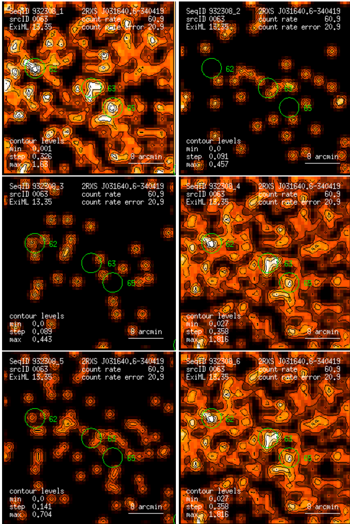
Figure 63: RASS 932308: detection 0063: band rate images, Gaussian filter: (1) PSPC channels 11 – 41, (2) 52 – 90, (3) 91 – 201, (4) 11 – 235, (5) 52 – 201, (6) 11 – 201. Broad band rates in counts/ks. Band rate contour levels in counts/ks/arcmin 2 .
