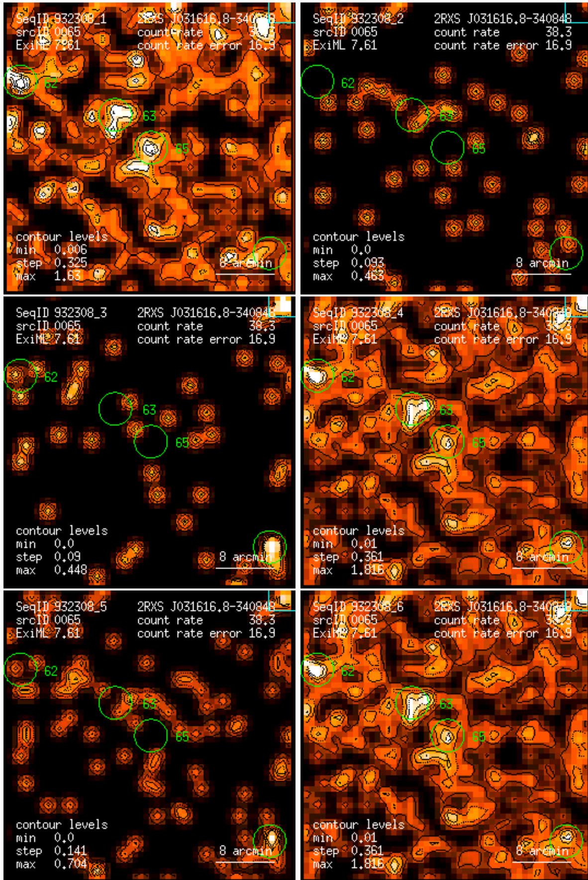
Figure 65: RASS 932308: detection 0065: band rate images, Gaussian filter: (1) PSPC channels 11 – 41, (2) 52 – 90, (3) 91 – 201, (4) 11 – 235, (5) 52 – 201, (6) 11 – 201. Broad band rates in counts/ks. Band rate contour levels in counts/ks/arcmin 2 .
