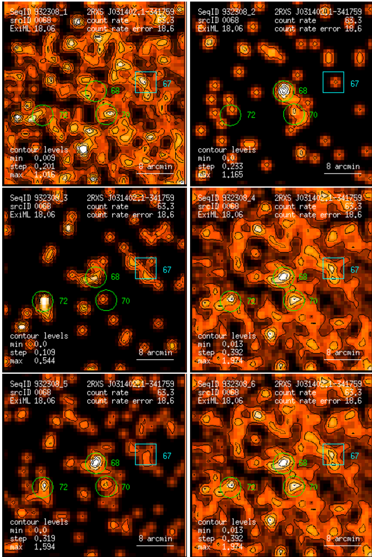
Figure 68: RASS 932308: detection 0068: band rate images, Gaussian filter: (1) PSPC channels 11 – 41, (2) 52 – 90, (3) 91 – 201, (4) 11 – 235, (5) 52 – 201, (6) 11 – 201. Broad band rates in counts/ks. Band rate contour levels in counts/ks/arcmin 2 .
