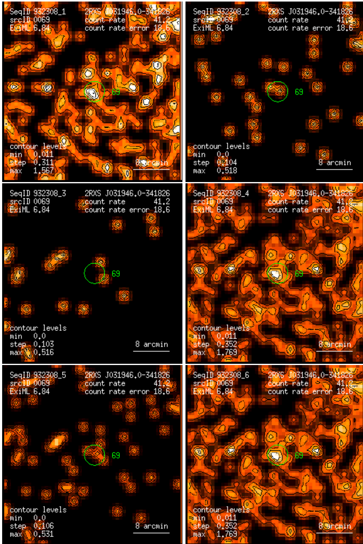
Figure 69: RASS 932308: detection 0069: band rate images, Gaussian filter: (1) PSPC channels 11 – 41, (2) 52 – 90, (3) 91 – 201, (4) 11 – 235, (5) 52 – 201, (6) 11 – 201. Broad band rates in counts/ks. Band rate contour levels in counts/ks/arcmin 2 .
