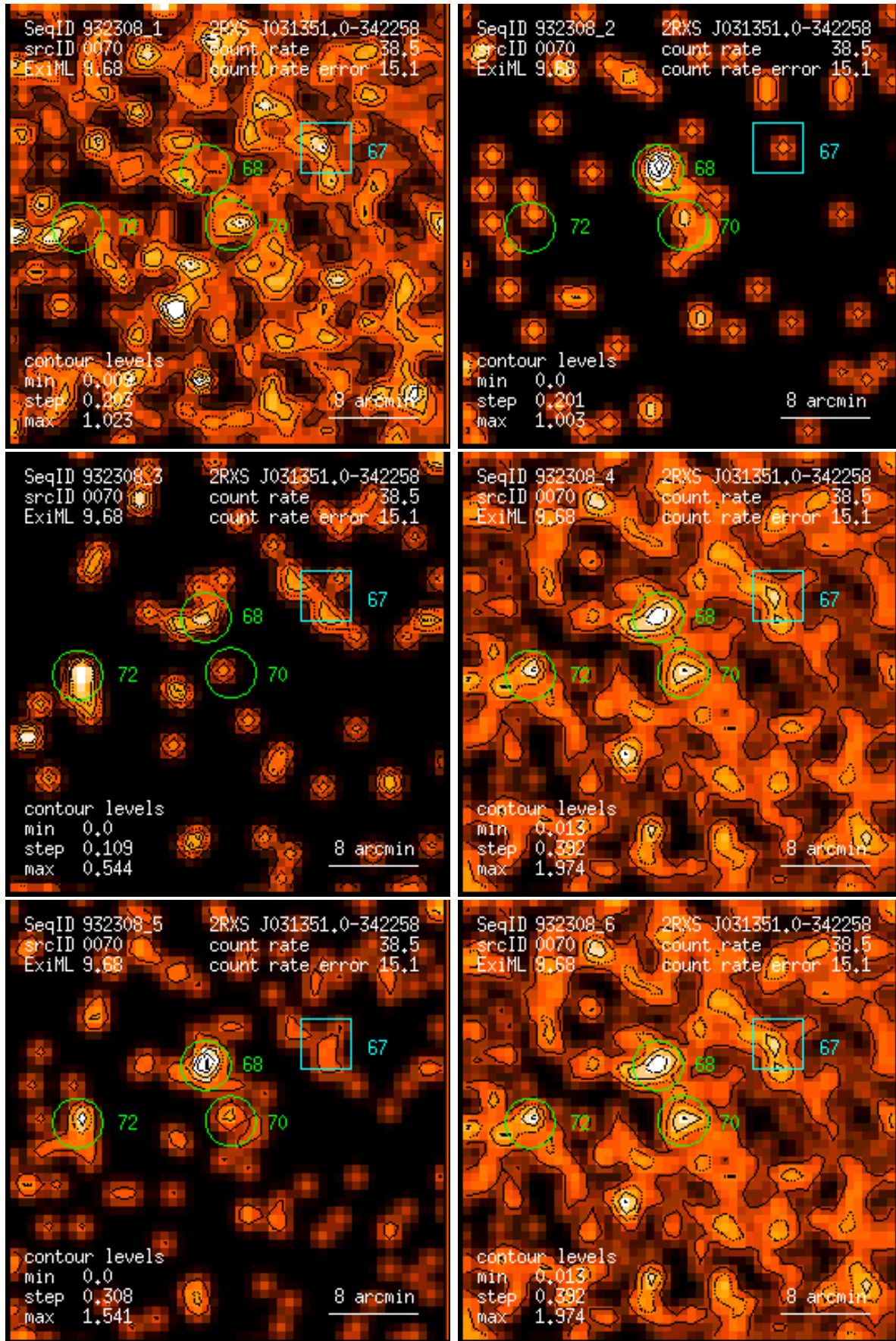
Figure 70: RASS 932308: detection 0070: band rate images, Gaussian filter: (1) PSPC channels 11 – 41, (2) 52 – 90, (3) 91 – 201, (4) 11 – 235, (5) 52 – 201, (6) 11 – 201. Broad band rates in counts/ks. Band rate contour levels in counts/ks/arcmin 2 .
