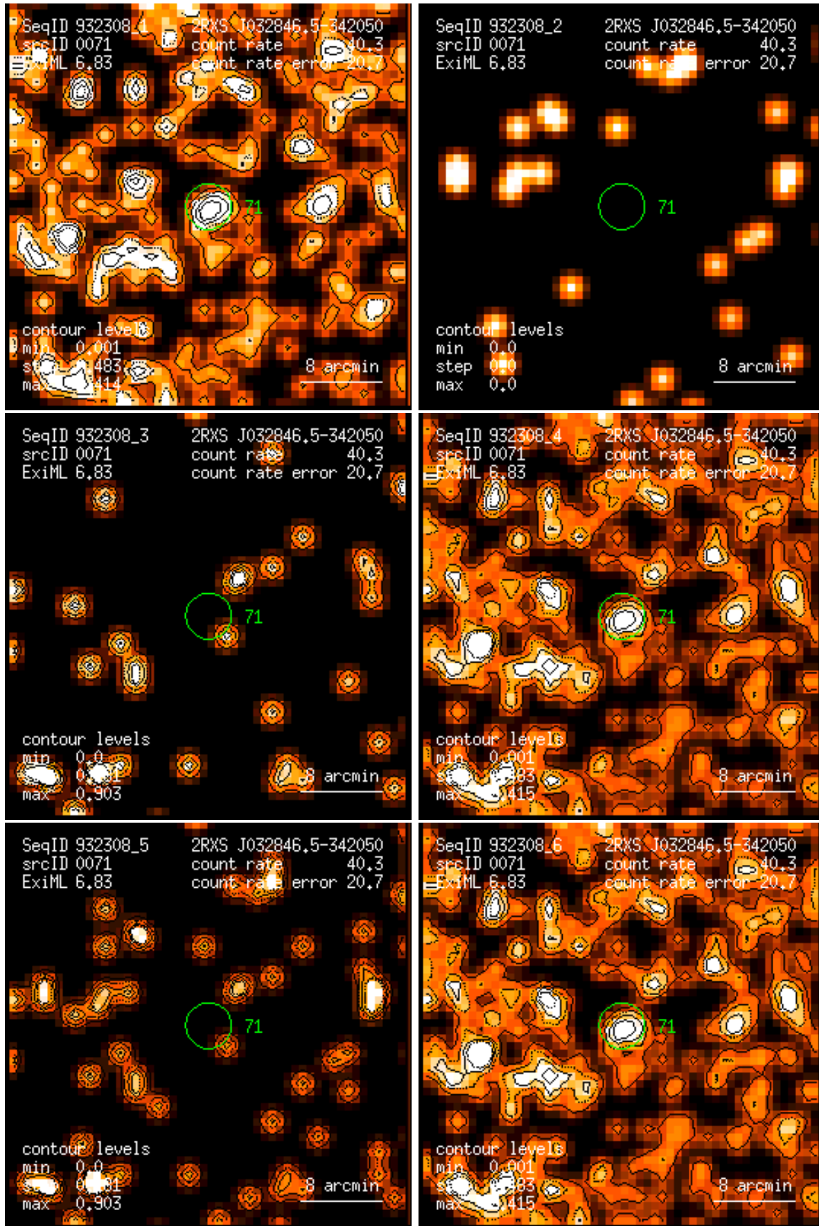
Figure 71: RASS 932308: detection 0071: band rate images, Gaussian filter: (1) PSPC channels 11 – 41, (2) 52 – 90, (3) 91 – 201, (4) 11 – 235, (5) 52 – 201, (6) 11 – 201. Broad band rates in counts/ks. Band rate contour levels in counts/ks/arcmin 2 .
