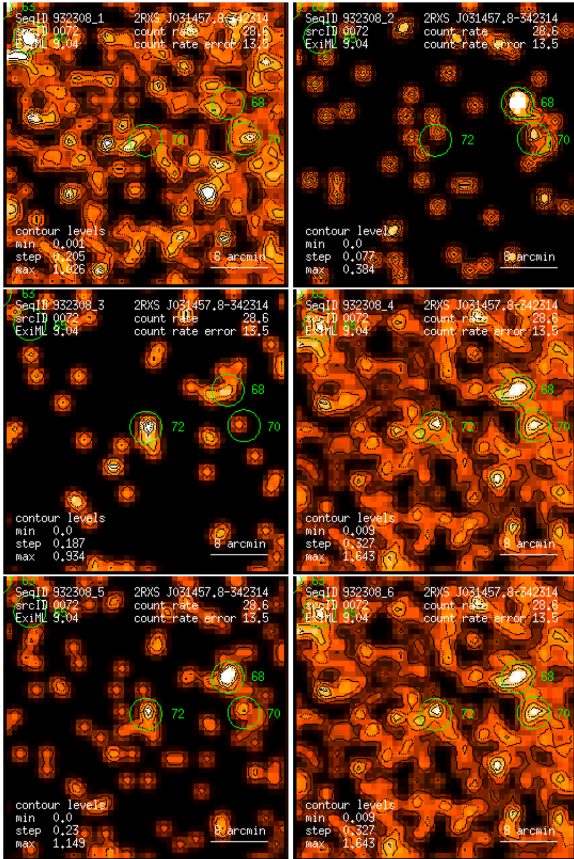
Figure 72: RASS 932308: detection 0072: band rate images, Gaussian filter: (1) PSPC channels 11 – 41, (2) 52 – 90, (3) 91 – 201, (4) 11 – 235, (5) 52 – 201, (6) 11 – 201. Broad band rates in counts/ks. Band rate contour levels in counts/ks/arcmin 2 .
