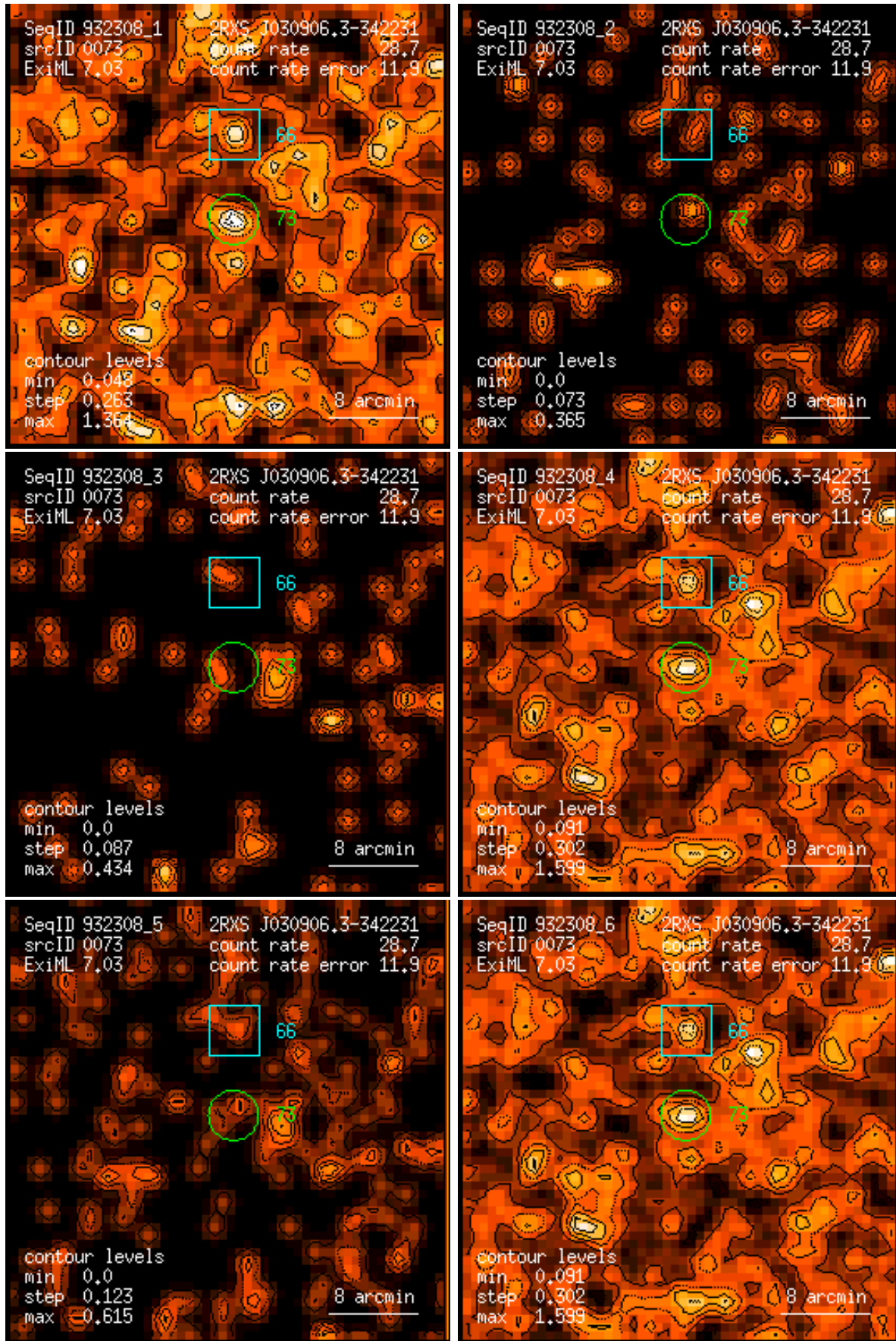
Figure 73: RASS 932308: detection 0073: band rate images, Gaussian filter: (1) PSPC channels 11 – 41, (2) 52 – 90, (3) 91 – 201, (4) 11 – 235, (5) 52 – 201, (6) 11 – 201. Broad band rates in counts/ks. Band rate contour levels in counts/ks/arcmin 2 .
